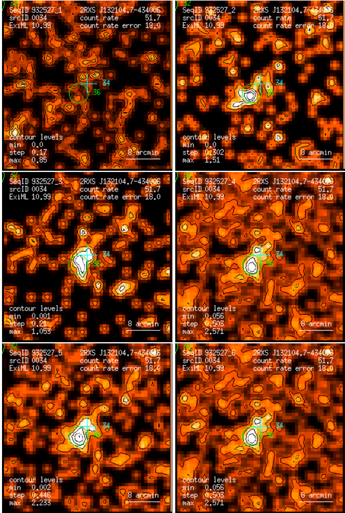
Figure 34: RASS 932527: detection 0034: band rate images, Gaussian filter: (1) PSPC channels 11 – 41, (2) 52 – 90, (3) 91 – 201, (4) 11 – 235, (5) 52 – 201, (6) 11 – 201. Broad band rates in counts/ks. Band rate contour levels in counts/ks/arcmin 2 .
