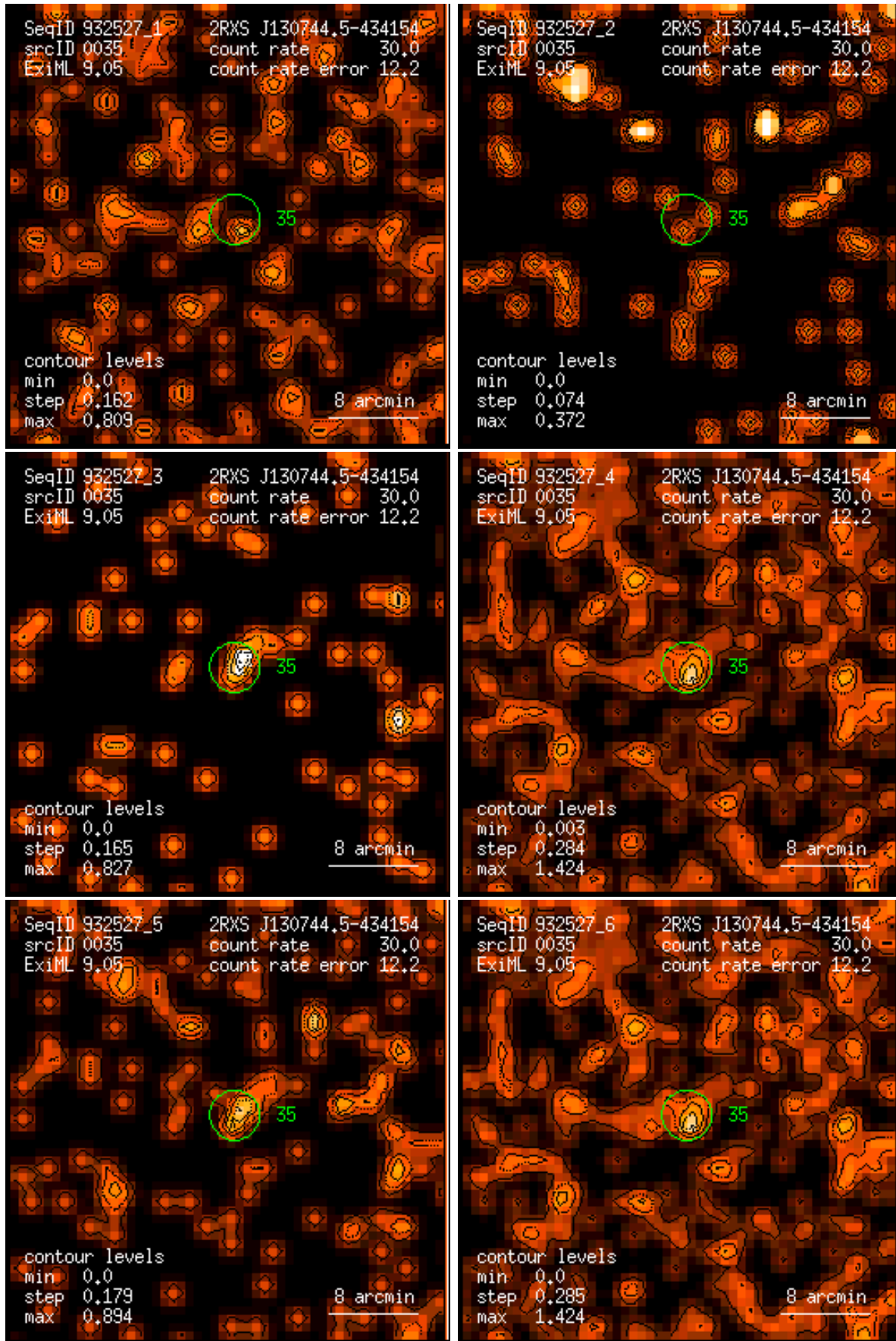
Figure 35: RASS 932527: detection 0035: band rate images, Gaussian filter: (1) PSPC channels 11 – 41, (2) 52 – 90, (3) 91 – 201, (4) 11 – 235, (5) 52 – 201, (6) 11 – 201. Broad band rates in counts/ks. Band rate contour levels in counts/ks/arcmin 2 .
