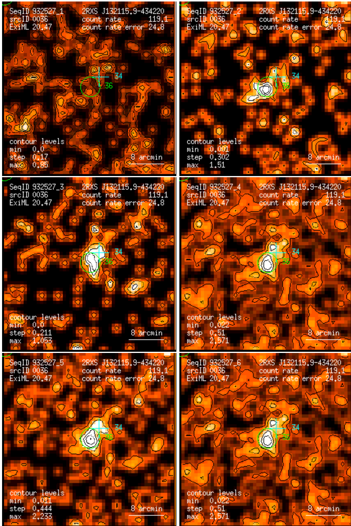
Figure 36: RASS 932527: detection 0036: band rate images, Gaussian filter: (1) PSPC channels 11 – 41, (2) 52 – 90, (3) 91 – 201, (4) 11 – 235, (5) 52 – 201, (6) 11 – 201. Broad band rates in counts/ks. Band rate contour levels in counts/ks/arcmin 2 .
