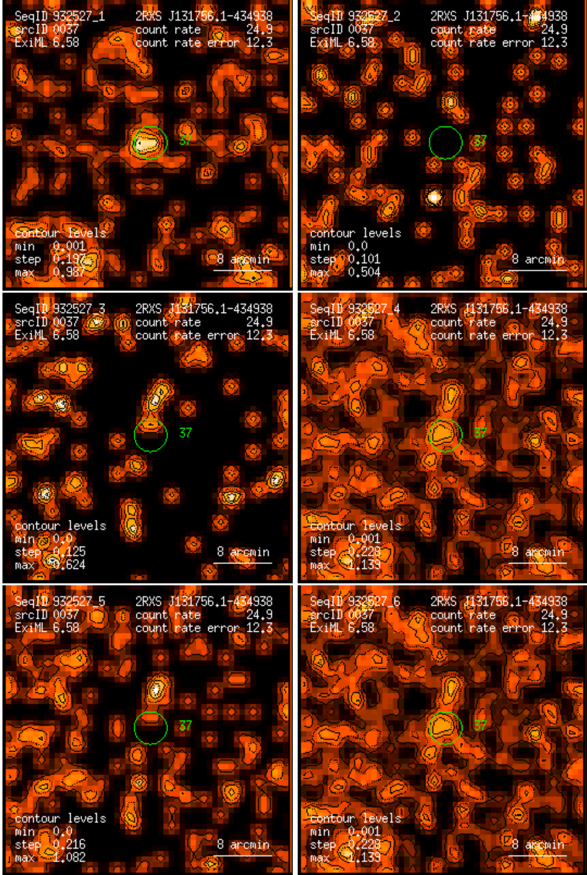
Figure 37: RASS 932527: detection 0037: band rate images, Gaussian filter: (1) PSPC channels 11 – 41, (2) 52 – 90, (3) 91 – 201, (4) 11 – 235, (5) 52 – 201, (6) 11 – 201. Broad band rates in counts/ks. Band rate contour levels in counts/ks/arcmin 2 .
