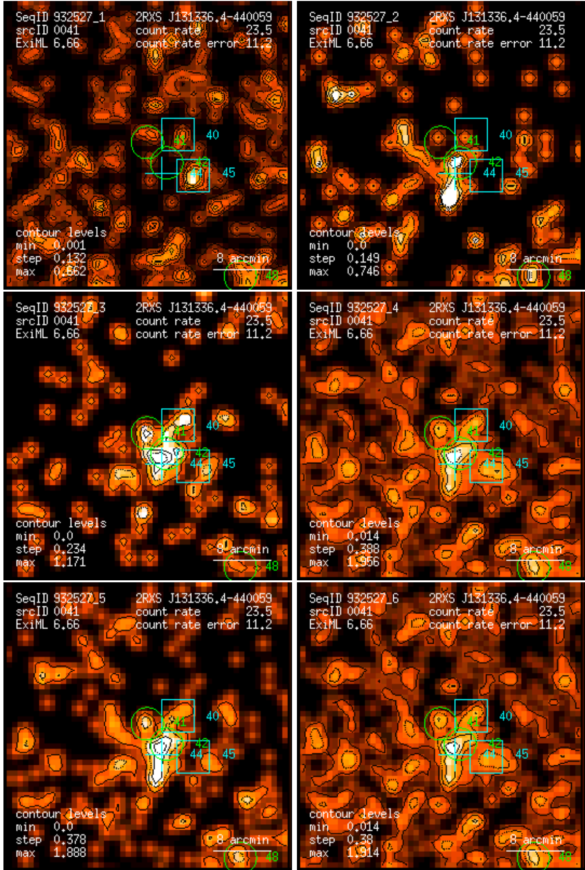
Figure 41: RASS 932527: detection 0041: band rate images, Gaussian filter: (1) PSPC channels 11 – 41, (2) 52 – 90, (3) 91 – 201, (4) 11 – 235, (5) 52 – 201, (6) 11 – 201. Broad band rates in counts/ks. Band rate contour levels in counts/ks/arcmin 2 .
