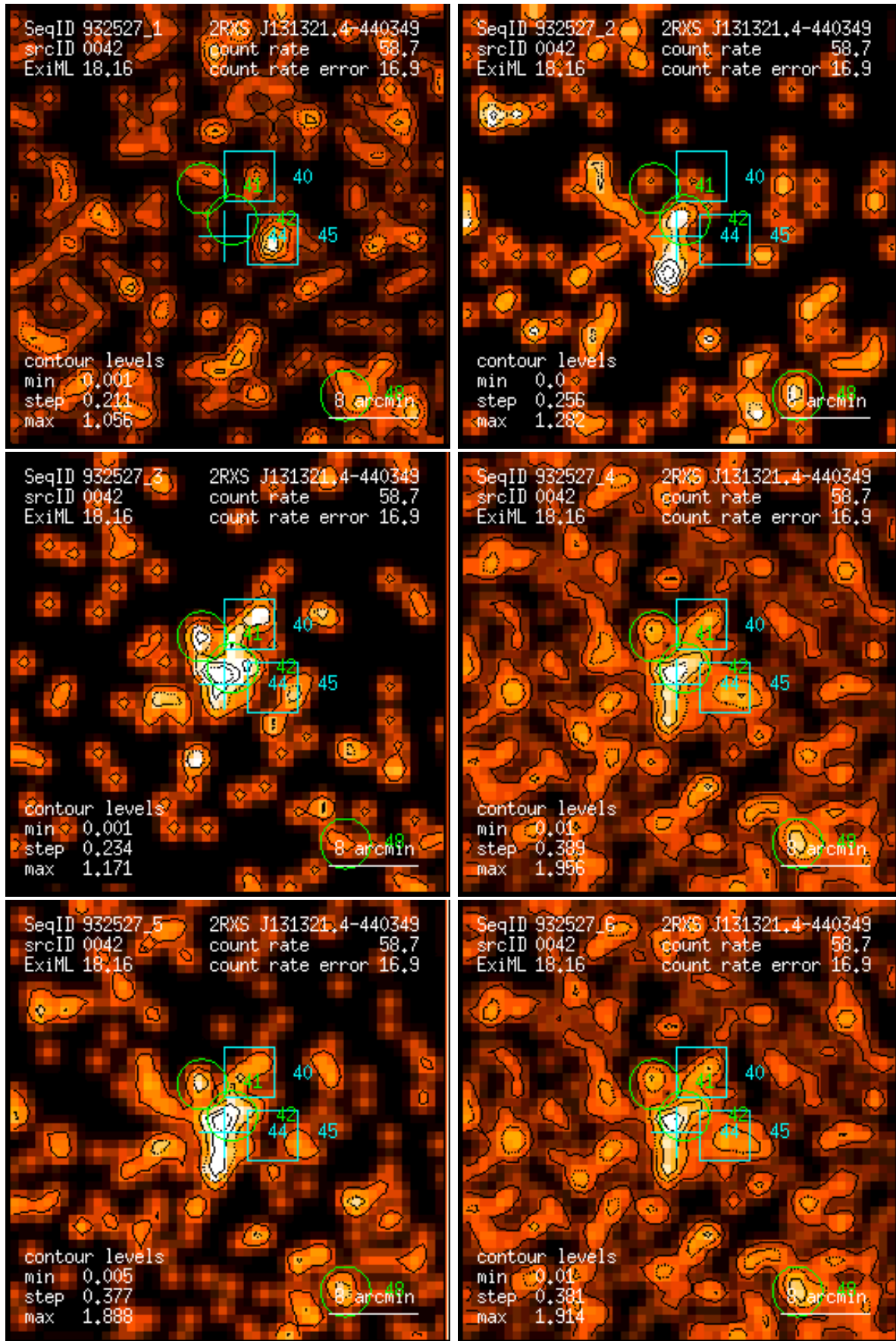
Figure 42: RASS 932527: detection 0042: band rate images, Gaussian filter: (1) PSPC channels 11 – 41, (2) 52 – 90, (3) 91 – 201, (4) 11 – 235, (5) 52 – 201, (6) 11 – 201. Broad band rates in counts/ks. Band rate contour levels in counts/ks/arcmin 2 .
