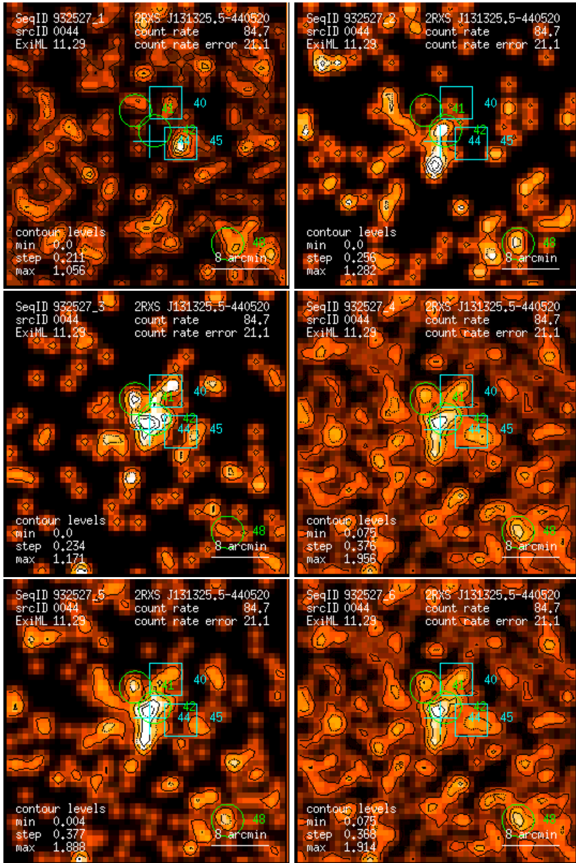
Figure 44: RASS 932527: detection 0044: band rate images, Gaussian filter: (1) PSPC channels 11 – 41, (2) 52 – 90, (3) 91 – 201, (4) 11 – 235, (5) 52 – 201, (6) 11 – 201. Broad band rates in counts/ks. Band rate contour levels in counts/ks/arcmin 2 .
