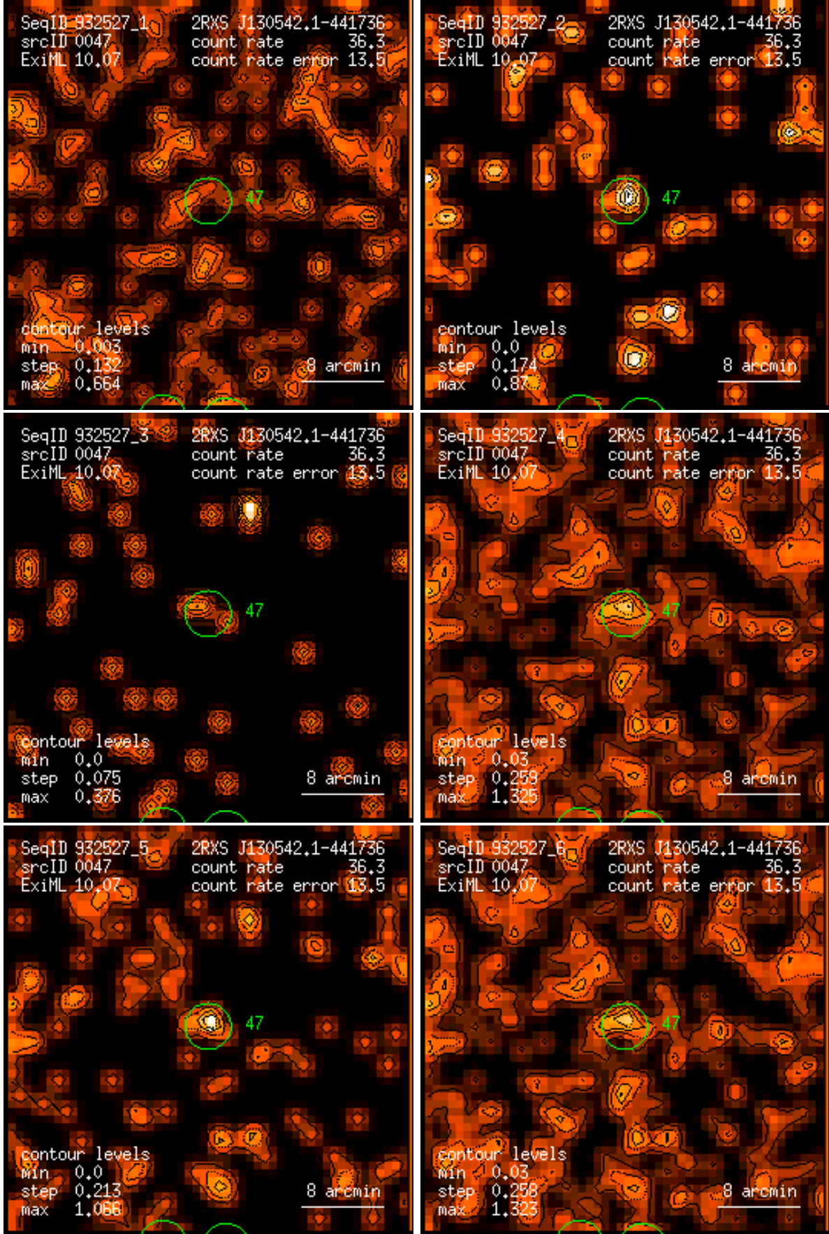
Figure 47: RASS 932527: detection 0047: band rate images, Gaussian filter: (1) PSPC channels 11 – 41, (2) 52 – 90, (3) 91 – 201, (4) 11 – 235, (5) 52 – 201, (6) 11 – 201. Broad band rates in counts/ks. Band rate contour levels in counts/ks/arcmin 2 .
