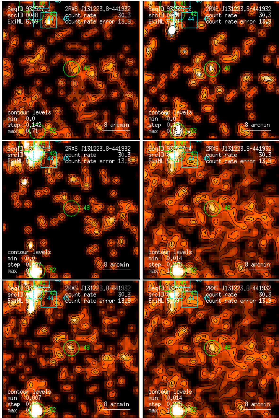
Figure 48: RASS 932527: detection 0048: band rate images, Gaussian filter: (1) PSPC channels 11 – 41, (2) 52 – 90, (3) 91 – 201, (4) 11 – 235, (5) 52 – 201, (6) 11 – 201. Broad band rates in counts/ks. Band rate contour levels in counts/ks/arcmin 2 .
