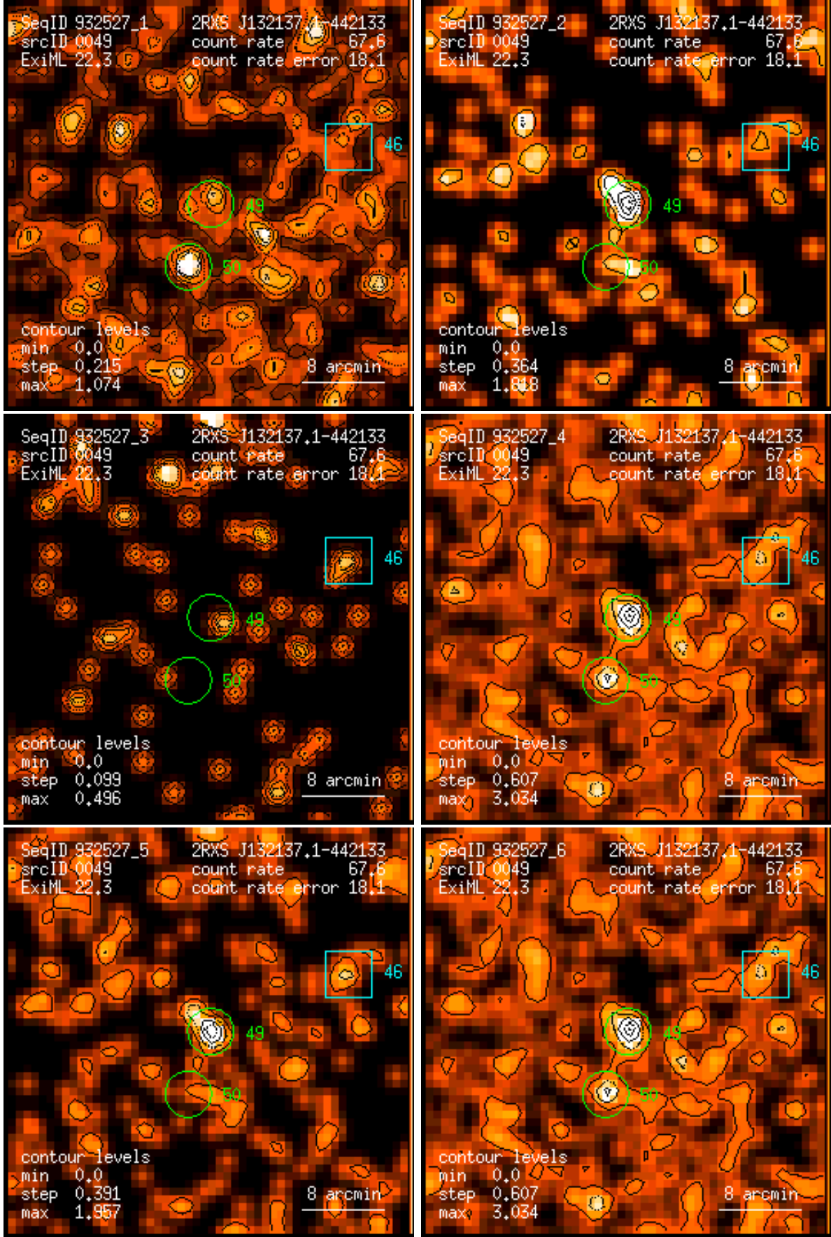
Figure 49: RASS 932527: detection 0049: band rate images, Gaussian filter: (1) PSPC channels 11 – 41, (2) 52 – 90, (3) 91 – 201, (4) 11 – 235, (5) 52 – 201, (6) 11 – 201. Broad band rates in counts/ks. Band rate contour levels in counts/ks/arcmin 2 .
