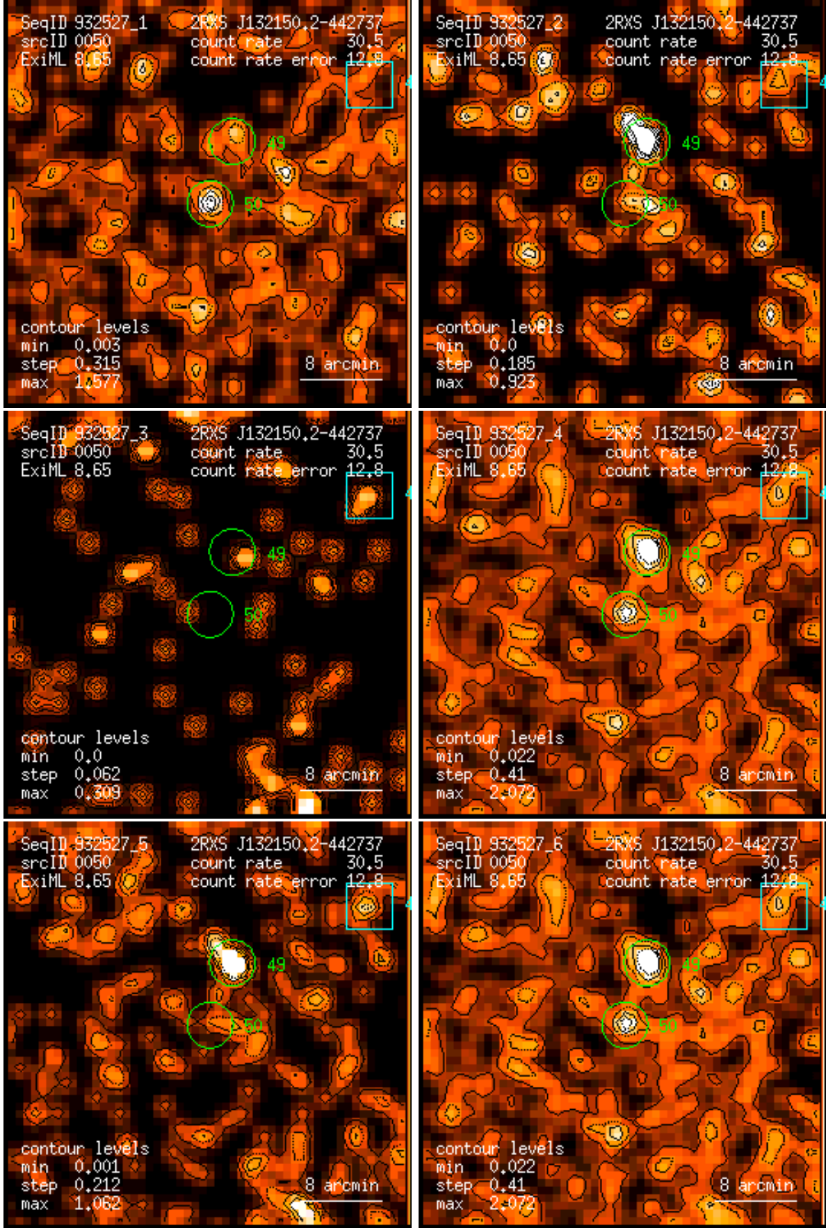
Figure 50: RASS 932527: detection 0050: band rate images, Gaussian filter: (1) PSPC channels 11 – 41, (2) 52 – 90, (3) 91 – 201, (4) 11 – 235, (5) 52 – 201, (6) 11 – 201. Broad band rates in counts/ks. Band rate contour levels in counts/ks/arcmin 2 .
