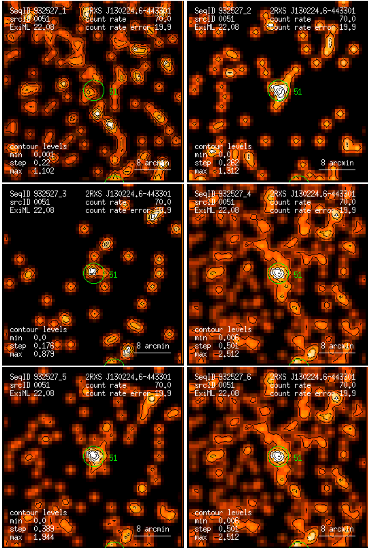
Figure 51: RASS 932527: detection 0051: band rate images, Gaussian filter: (1) PSPC channels 11 – 41, (2) 52 – 90, (3) 91 – 201, (4) 11 – 235, (5) 52 – 201, (6) 11 – 201. Broad band rates in counts/ks. Band rate contour levels in counts/ks/arcmin 2 .
