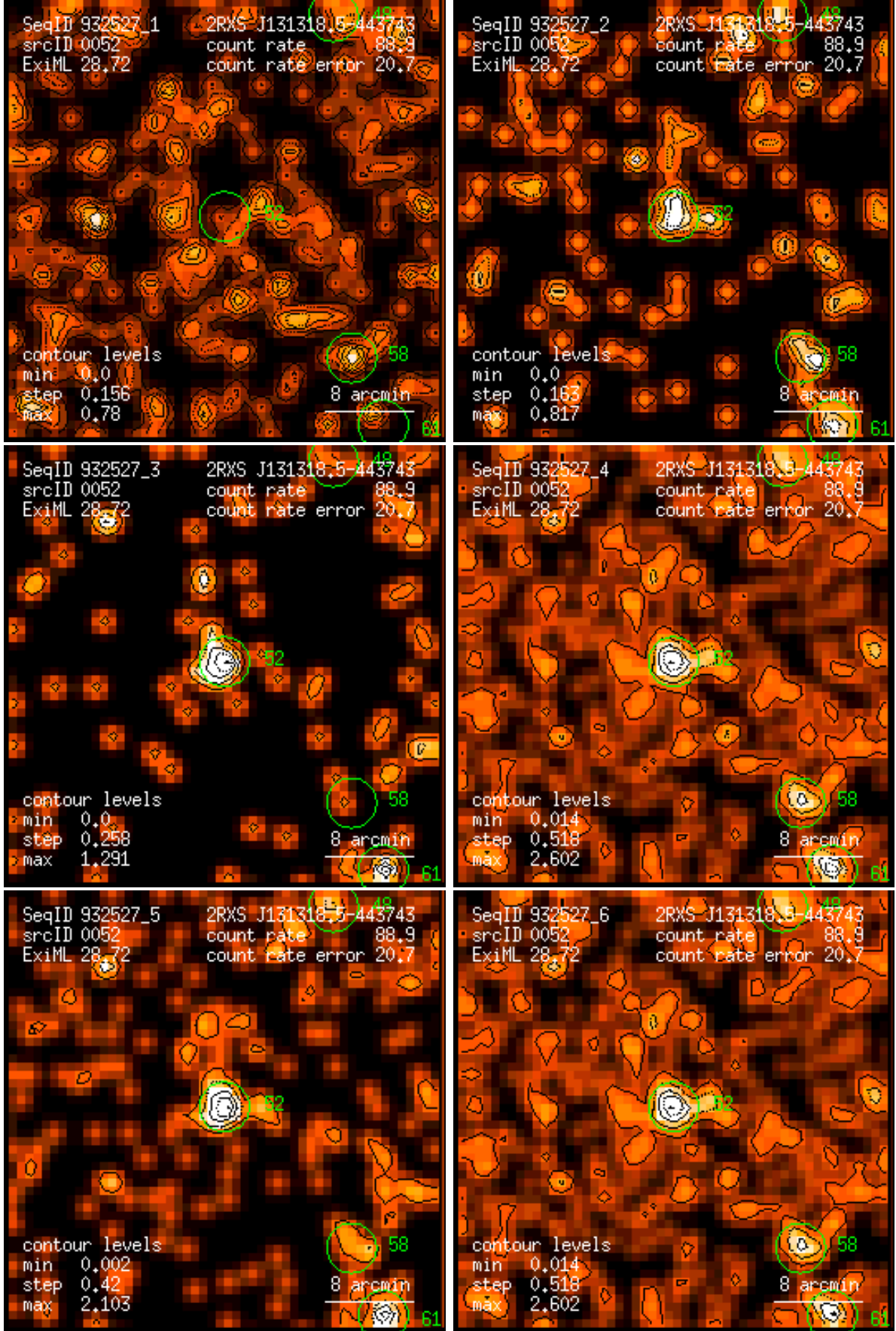
Figure 52: RASS 932527: detection 0052: band rate images, Gaussian filter: (1) PSPC channels 11 – 41, (2) 52 – 90, (3) 91 – 201, (4) 11 – 235, (5) 52 – 201, (6) 11 – 201. Broad band rates in counts/ks. Band rate contour levels in counts/ks/arcmin 2 .
