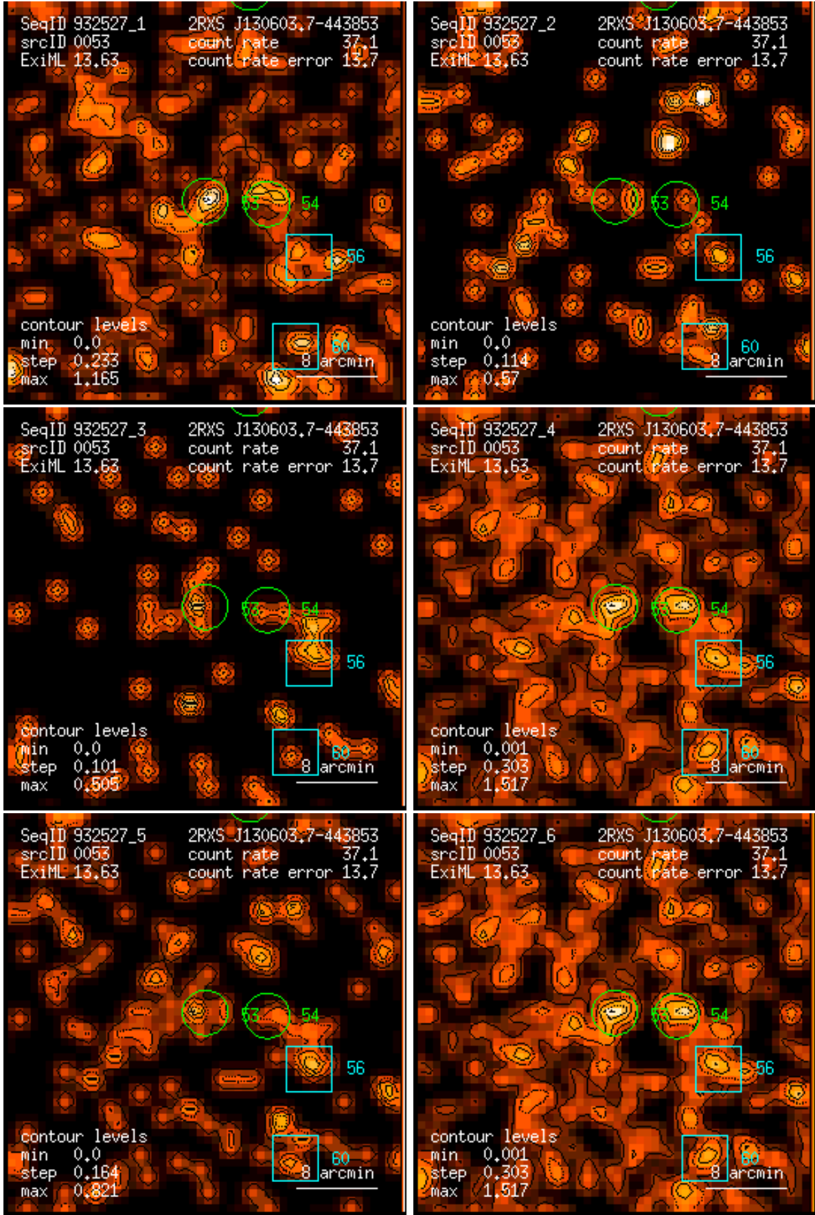
Figure 53: RASS 932527: detection 0053: band rate images, Gaussian filter: (1) PSPC channels 11 – 41, (2) 52 – 90, (3) 91 – 201, (4) 11 – 235, (5) 52 – 201, (6) 11 – 201. Broad band rates in counts/ks. Band rate contour levels in counts/ks/arcmin 2 .
