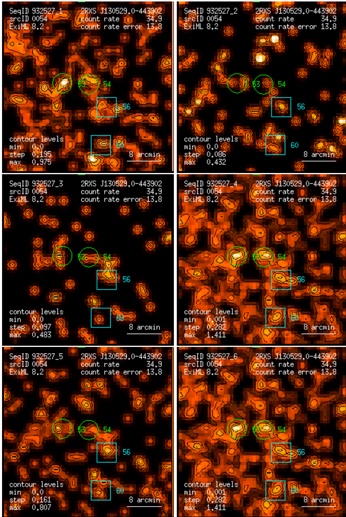
Figure 54: RASS 932527: detection 0054: band rate images, Gaussian filter: (1) PSPC channels 11 – 41, (2) 52 – 90, (3) 91 – 201, (4) 11 – 235, (5) 52 – 201, (6) 11 – 201. Broad band rates in counts/ks. Band rate contour levels in counts/ks/arcmin 2 .
