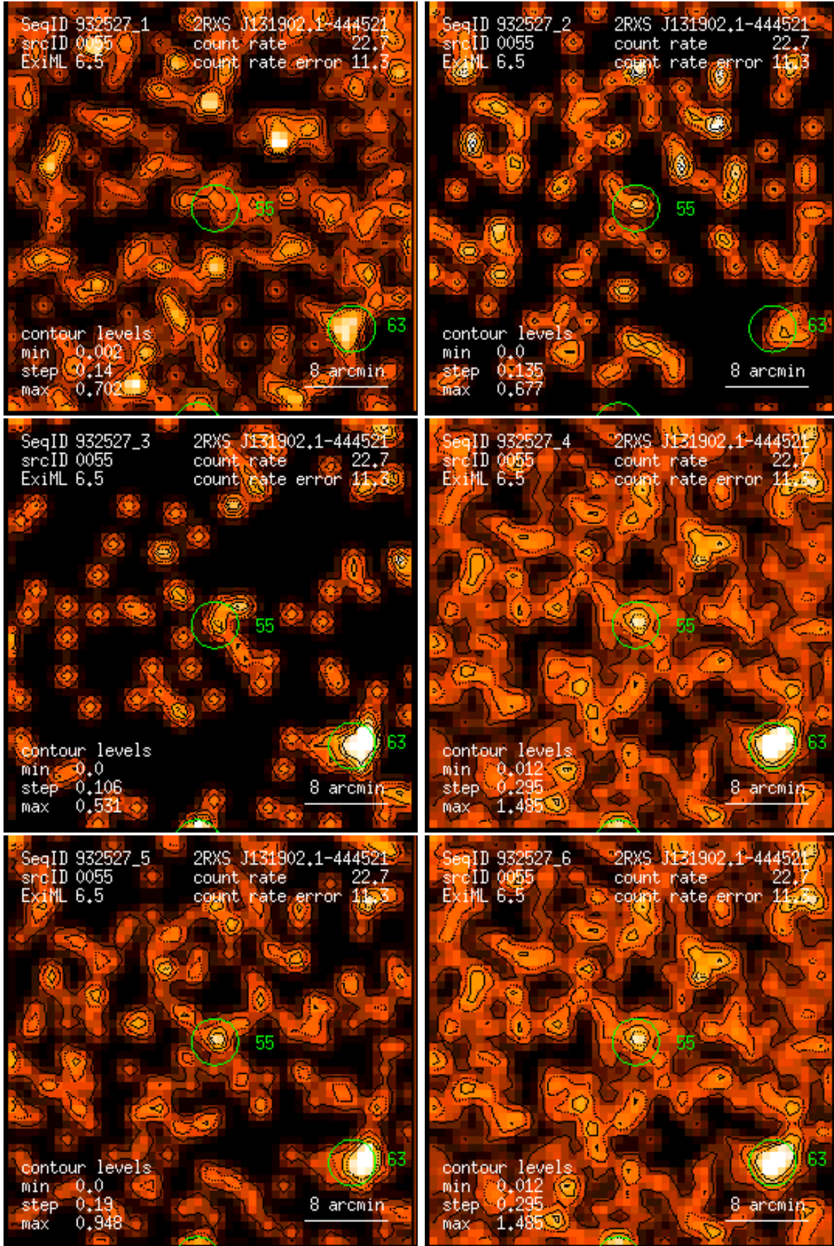
Figure 55: RASS 932527: detection 0055: band rate images, Gaussian filter: (1) PSPC channels 11 – 41, (2) 52 – 90, (3) 91 – 201, (4) 11 – 235, (5) 52 – 201, (6) 11 – 201. Broad band rates in counts/ks. Band rate contour levels in counts/ks/arcmin 2 .
