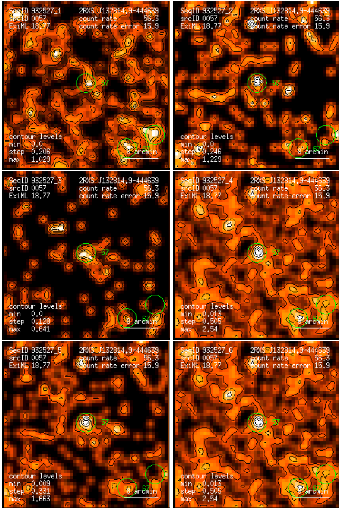
Figure 57: RASS 932527: detection 0057: band rate images, Gaussian filter: (1) PSPC channels 11 – 41, (2) 52 – 90, (3) 91 – 201, (4) 11 – 235, (5) 52 – 201, (6) 11 – 201. Broad band rates in counts/ks. Band rate contour levels in counts/ks/arcmin 2 .
