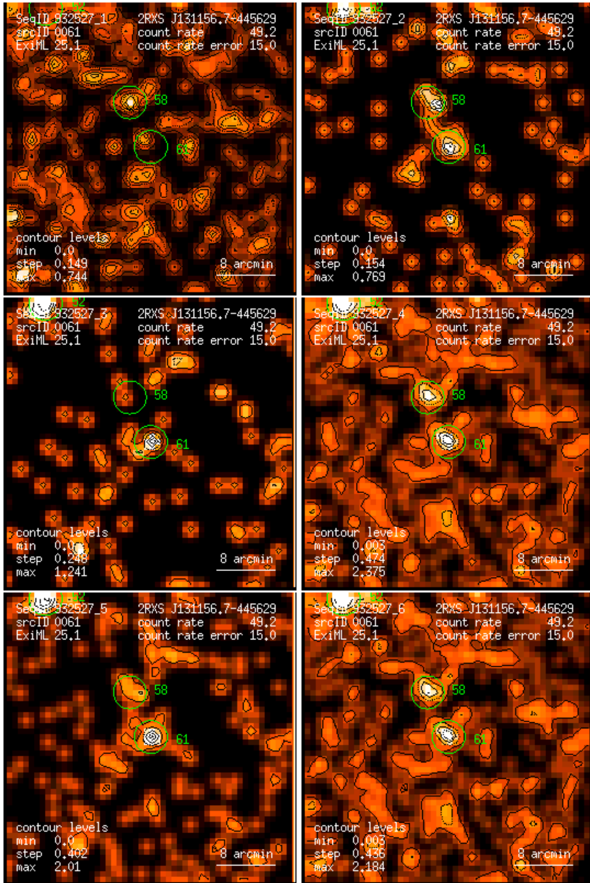
Figure 61: RASS 932527: detection 0061: band rate images, Gaussian filter: (1) PSPC channels 11 – 41, (2) 52 – 90, (3) 91 – 201, (4) 11 – 235, (5) 52 – 201, (6) 11 – 201. Broad band rates in counts/ks. Band rate contour levels in counts/ks/arcmin 2 .
