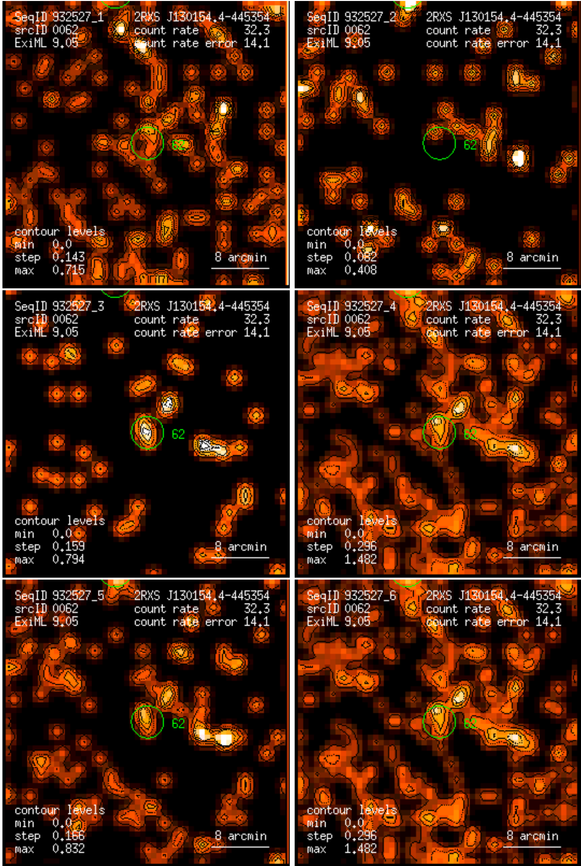
Figure 62: RASS 932527: detection 0062: band rate images, Gaussian filter: (1) PSPC channels 11 – 41, (2) 52 – 90, (3) 91 – 201, (4) 11 – 235, (5) 52 – 201, (6) 11 – 201. Broad band rates in counts/ks. Band rate contour levels in counts/ks/arcmin 2 .
