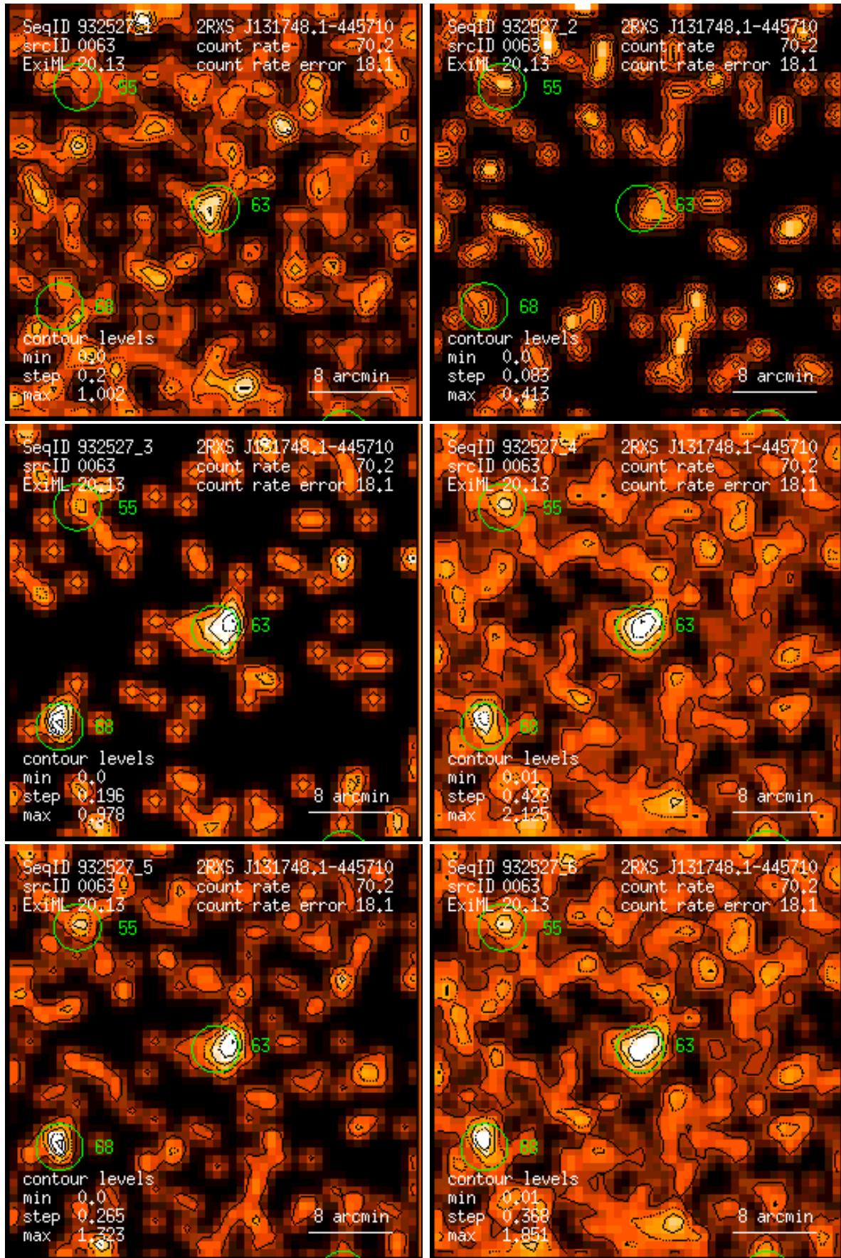
Figure 63: RASS 932527: detection 0063: band rate images, Gaussian filter: (1) PSPC channels 11 – 41, (2) 52 – 90, (3) 91 – 201, (4) 11 – 235, (5) 52 – 201, (6) 11 – 201. Broad band rates in counts/ks. Band rate contour levels in counts/ks/arcmin 2 .
