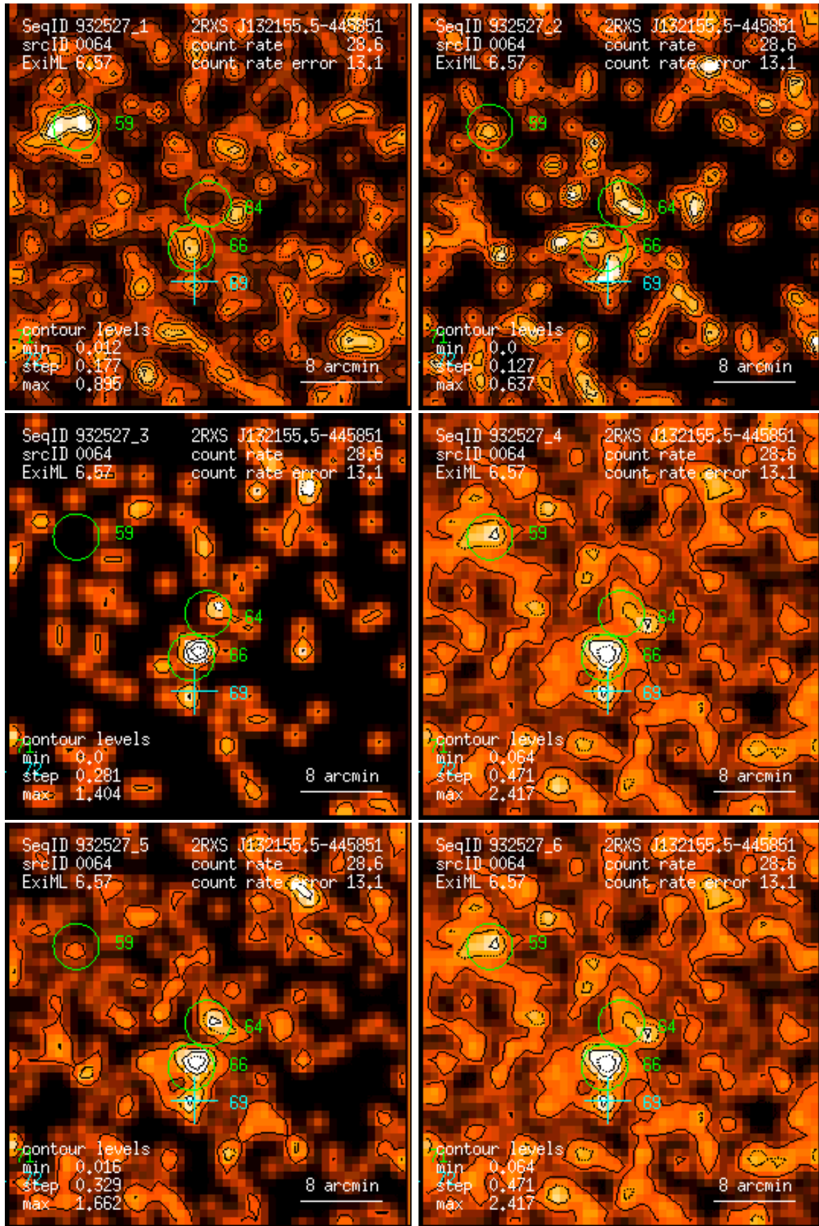
Figure 64: RASS 932527: detection 0064: band rate images, Gaussian filter: (1) PSPC channels 11 – 41, (2) 52 – 90, (3) 91 – 201, (4) 11 – 235, (5) 52 – 201, (6) 11 – 201. Broad band rates in counts/ks. Band rate contour levels in counts/ks/arcmin 2 .
