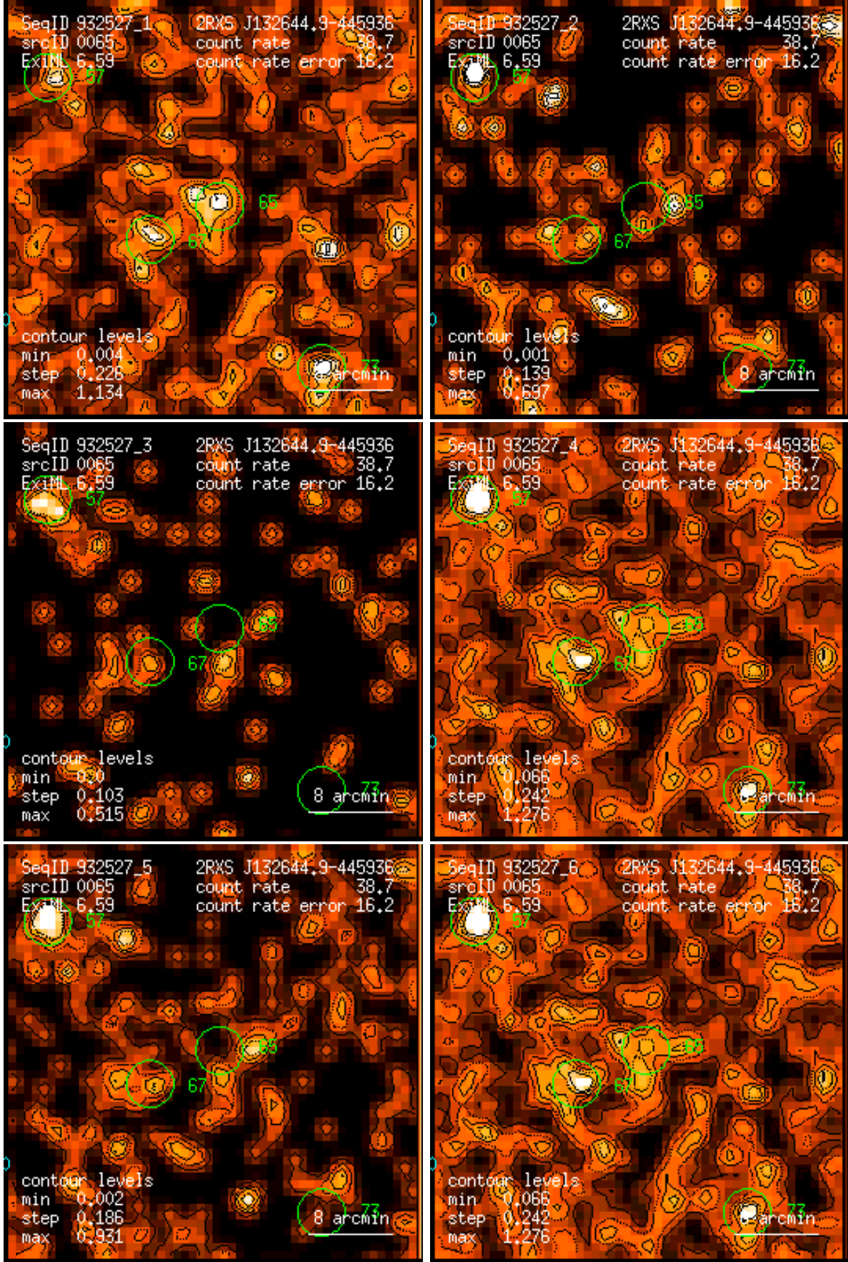
Figure 65: RASS 932527: detection 0065: band rate images, Gaussian filter: (1) PSPC channels 11 – 41, (2) 52 – 90, (3) 91 – 201, (4) 11 – 235, (5) 52 – 201, (6) 11 – 201. Broad band rates in counts/ks. Band rate contour levels in counts/ks/arcmin 2 .
