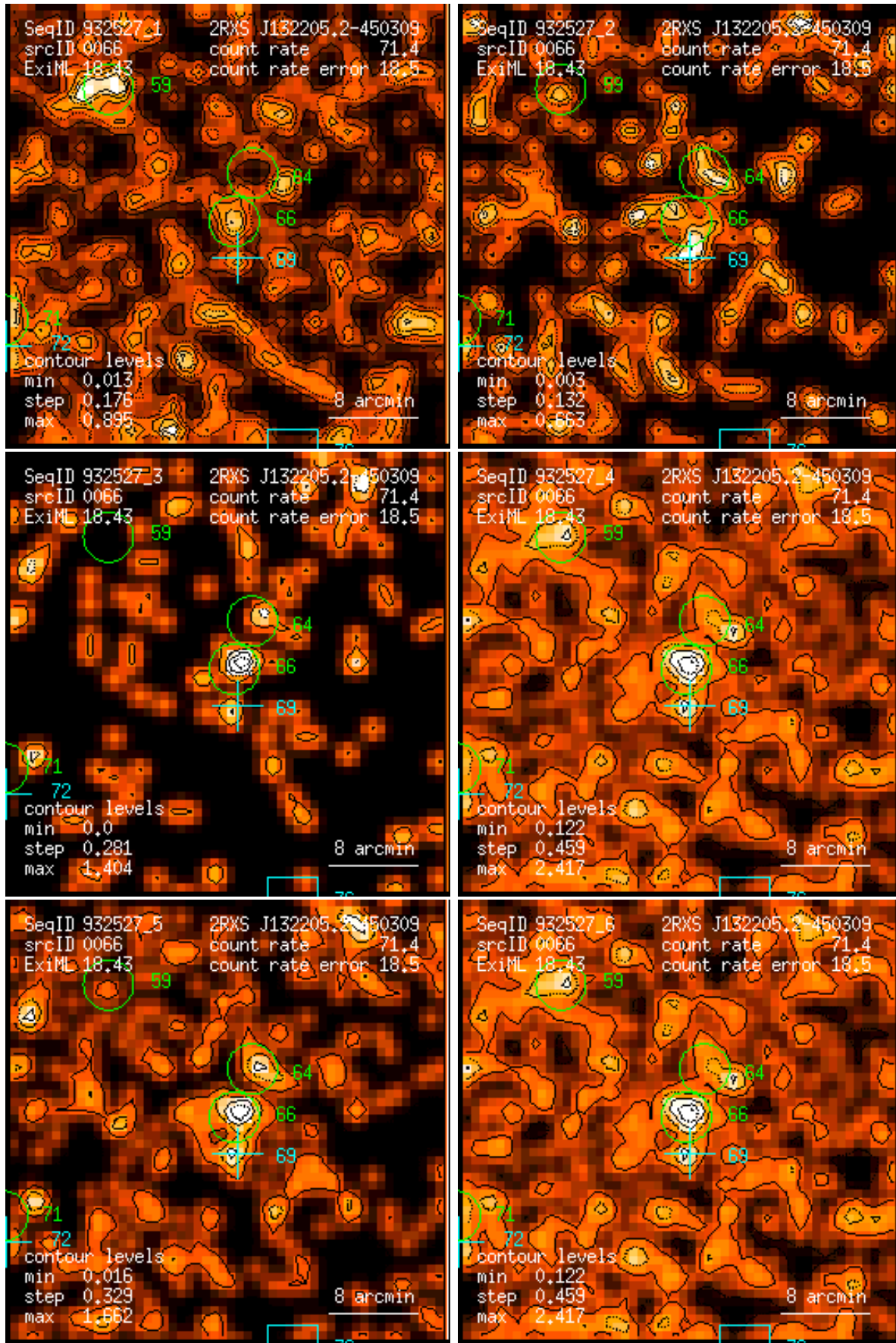
Figure 66: RASS 932527: detection 0066: band rate images, Gaussian filter: (1) PSPC channels 11 – 41, (2) 52 – 90, (3) 91 – 201, (4) 11 – 235, (5) 52 – 201, (6) 11 – 201. Broad band rates in counts/ks. Band rate contour levels in counts/ks/arcmin 2 .
