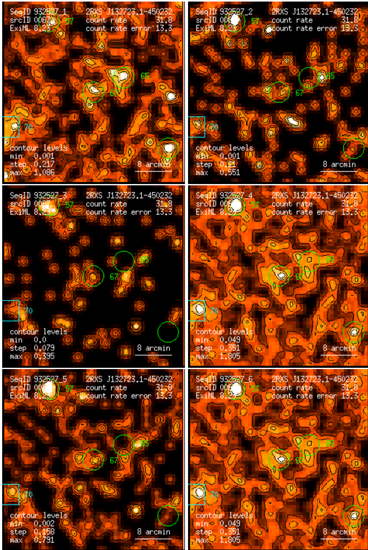
Figure 67: RASS 932527: detection 0067: band rate images, Gaussian filter: (1) PSPC channels 11 – 41, (2) 52 – 90, (3) 91 – 201, (4) 11 – 235, (5) 52 – 201, (6) 11 – 201. Broad band rates in counts/ks. Band rate contour levels in counts/ks/arcmin 2 .
