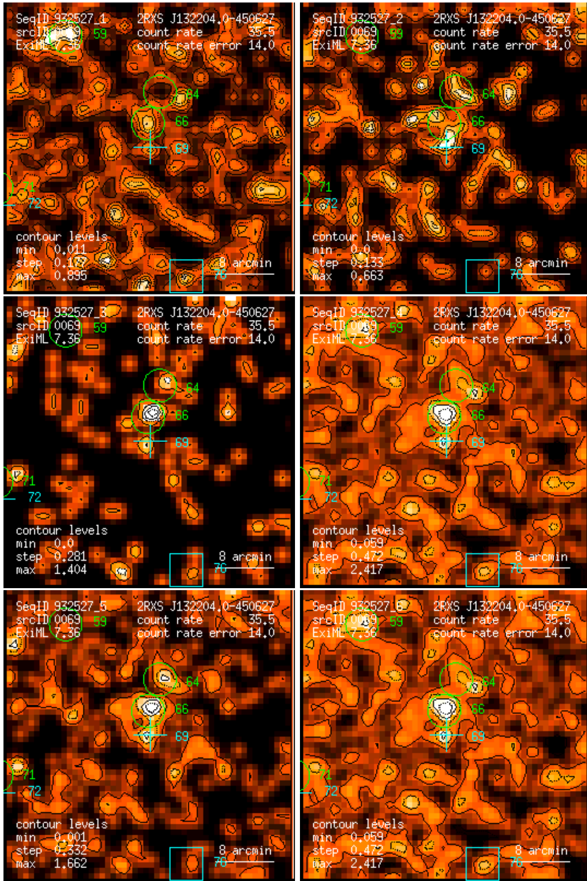
Figure 69: RASS 932527: detection 0069: band rate images, Gaussian filter: (1) PSPC channels 11 – 41, (2) 52 – 90, (3) 91 – 201, (4) 11 – 235, (5) 52 – 201, (6) 11 – 201. Broad band rates in counts/ks. Band rate contour levels in counts/ks/arcmin 2 .
