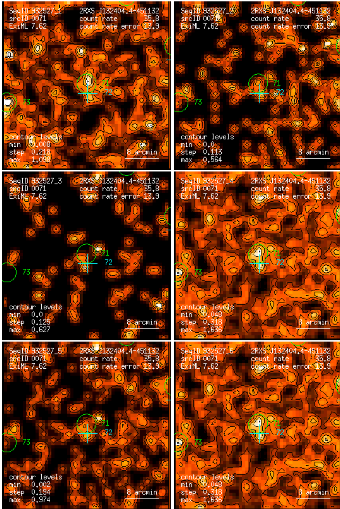
Figure 71: RASS 932527: detection 0071: band rate images, Gaussian filter: (1) PSPC channels 11 – 41, (2) 52 – 90, (3) 91 – 201, (4) 11 – 235, (5) 52 – 201, (6) 11 – 201. Broad band rates in counts/ks. Band rate contour levels in counts/ks/arcmin 2 .
