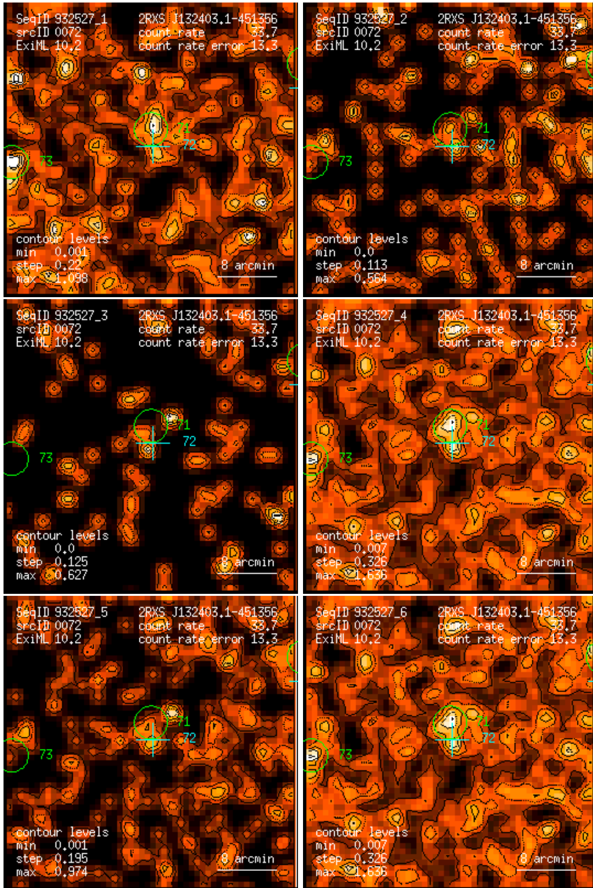
Figure 72: RASS 932527: detection 0072: band rate images, Gaussian filter: (1) PSPC channels 11 – 41, (2) 52 – 90, (3) 91 – 201, (4) 11 – 235, (5) 52 – 201, (6) 11 – 201. Broad band rates in counts/ks. Band rate contour levels in counts/ks/arcmin 2 .
