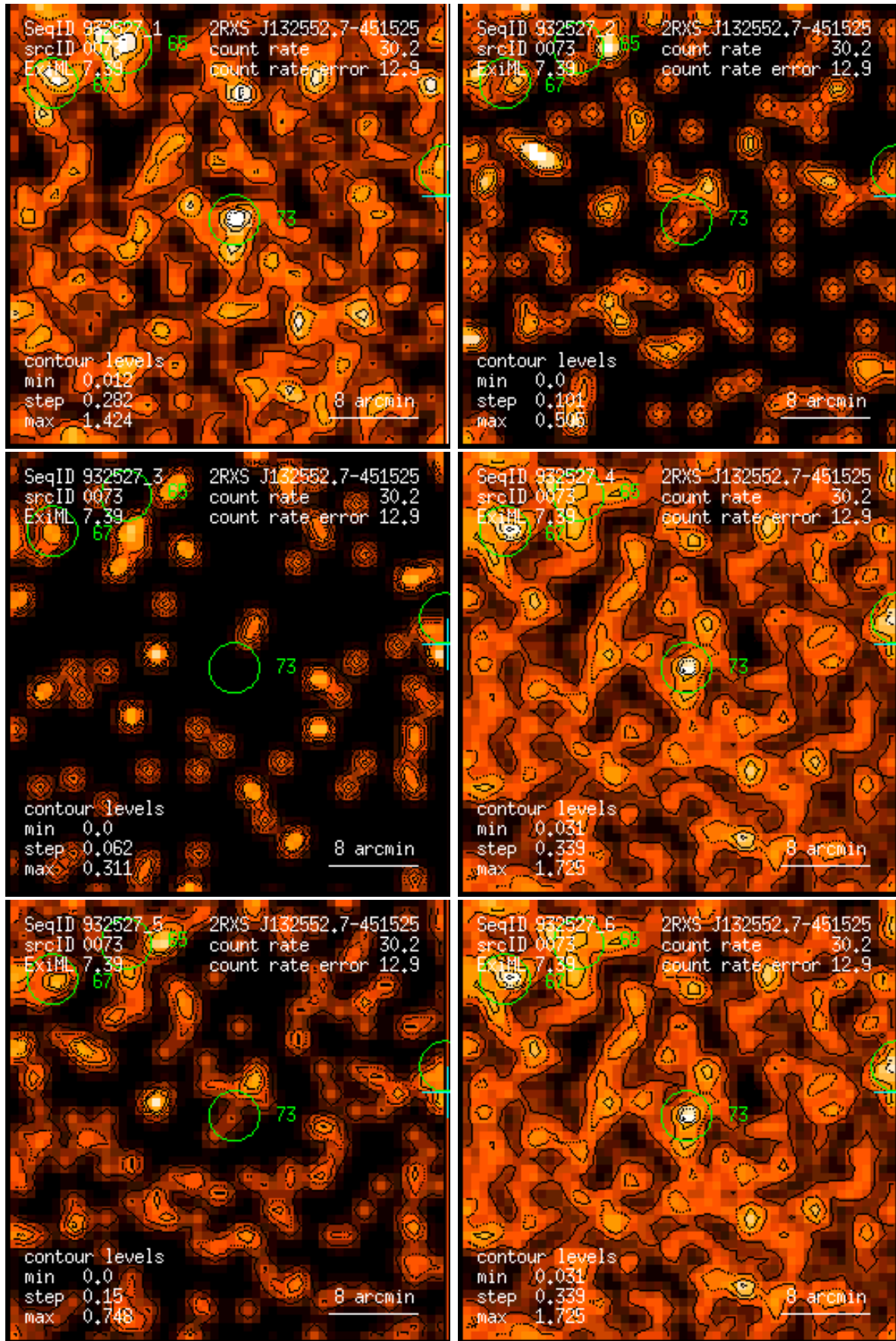
Figure 73: RASS 932527: detection 0073: band rate images, Gaussian filter: (1) PSPC channels 11 – 41, (2) 52 – 90, (3) 91 – 201, (4) 11 – 235, (5) 52 – 201, (6) 11 – 201. Broad band rates in counts/ks. Band rate contour levels in counts/ks/arcmin 2 .
