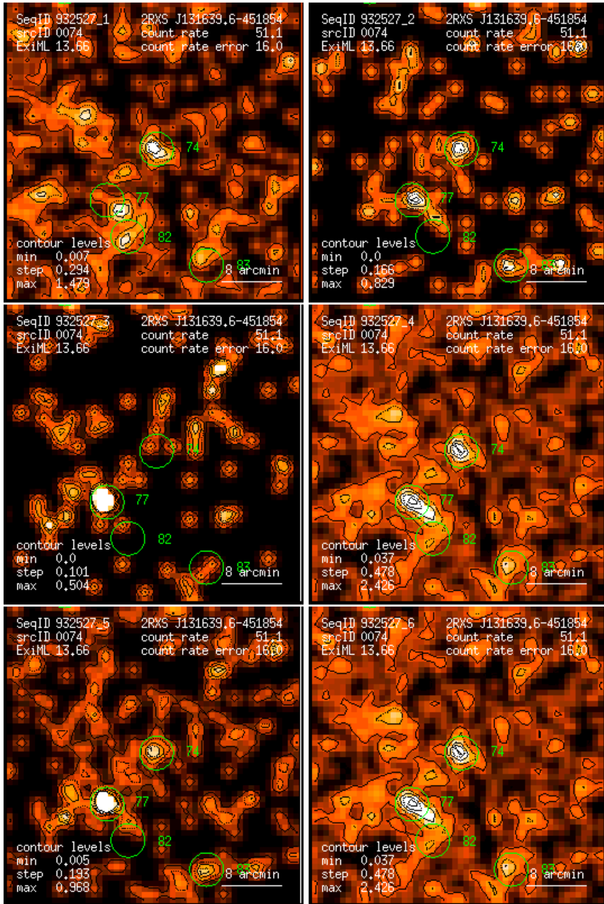
Figure 74: RASS 932527: detection 0074: band rate images, Gaussian filter: (1) PSPC channels 11 – 41, (2) 52 – 90, (3) 91 – 201, (4) 11 – 235, (5) 52 – 201, (6) 11 – 201. Broad band rates in counts/ks. Band rate contour levels in counts/ks/arcmin 2 .
