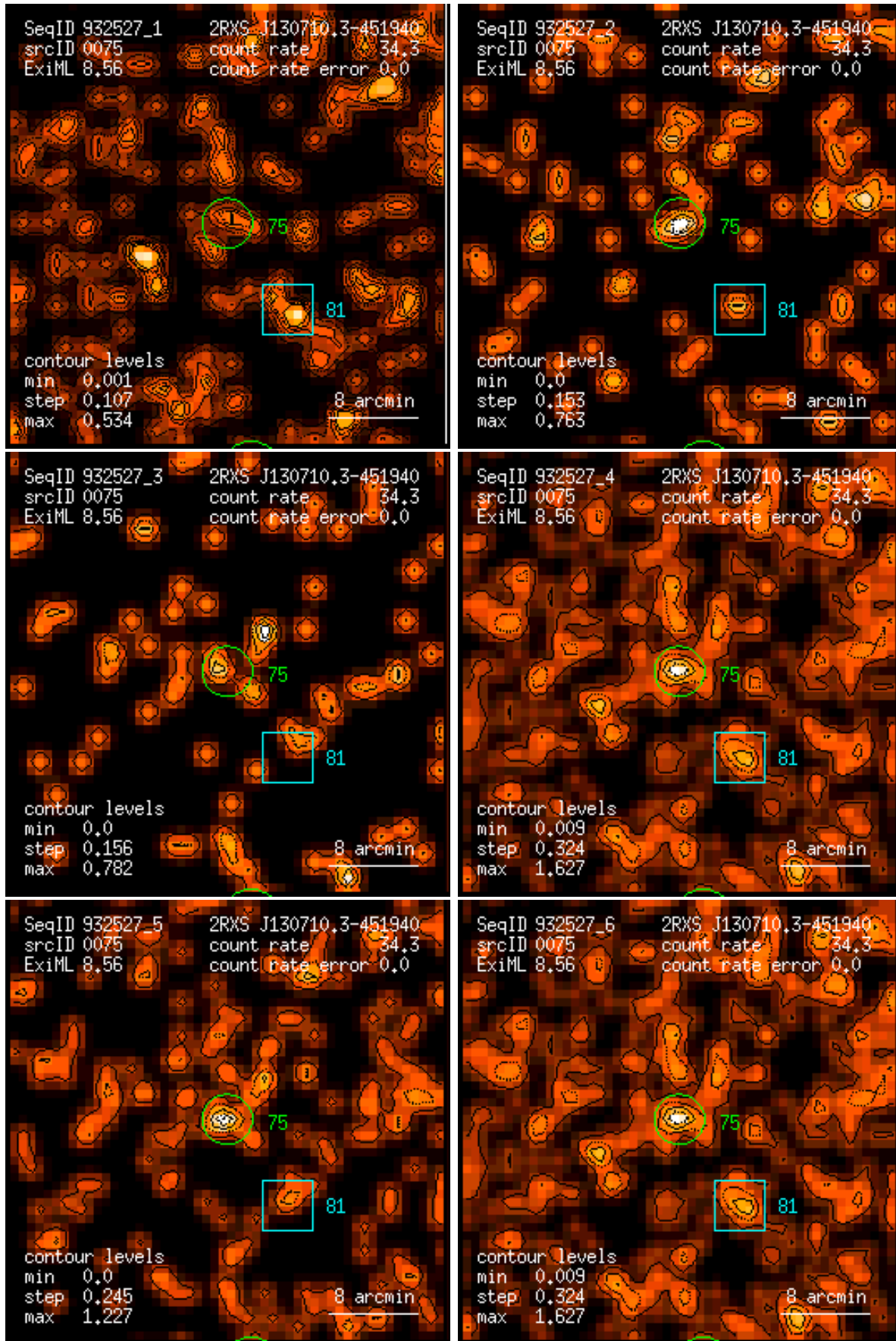
Figure 75: RASS 932527: detection 0075: band rate images, Gaussian filter: (1) PSPC channels 11 – 41, (2) 52 – 90, (3) 91 – 201, (4) 11 – 235, (5) 52 – 201, (6) 11 – 201. Broad band rates in counts/ks. Band rate contour levels in counts/ks/arcmin 2 .
