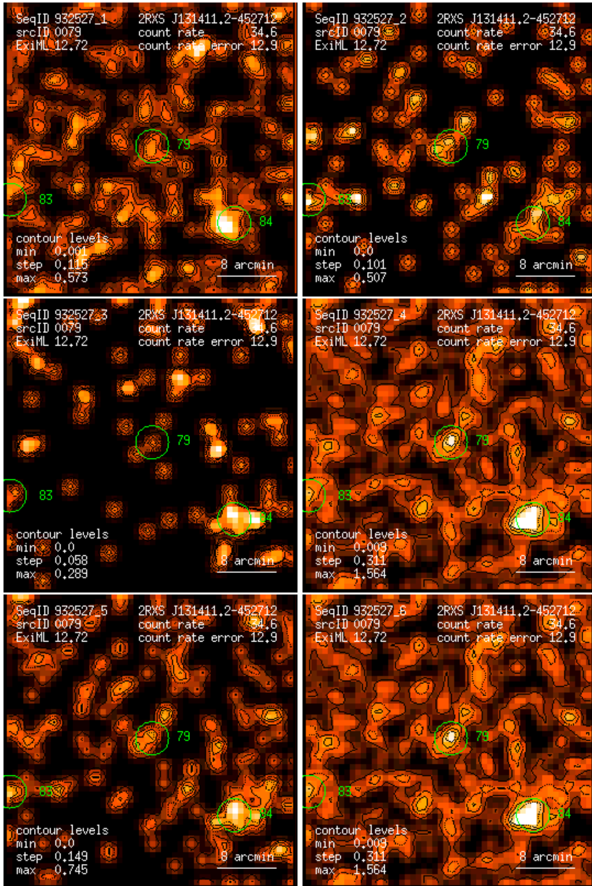
Figure 79: RASS 932527: detection 0079: band rate images, Gaussian filter: (1) PSPC channels 11 – 41, (2) 52 – 90, (3) 91 – 201, (4) 11 – 235, (5) 52 – 201, (6) 11 – 201. Broad band rates in counts/ks. Band rate contour levels in counts/ks/arcmin 2 .
