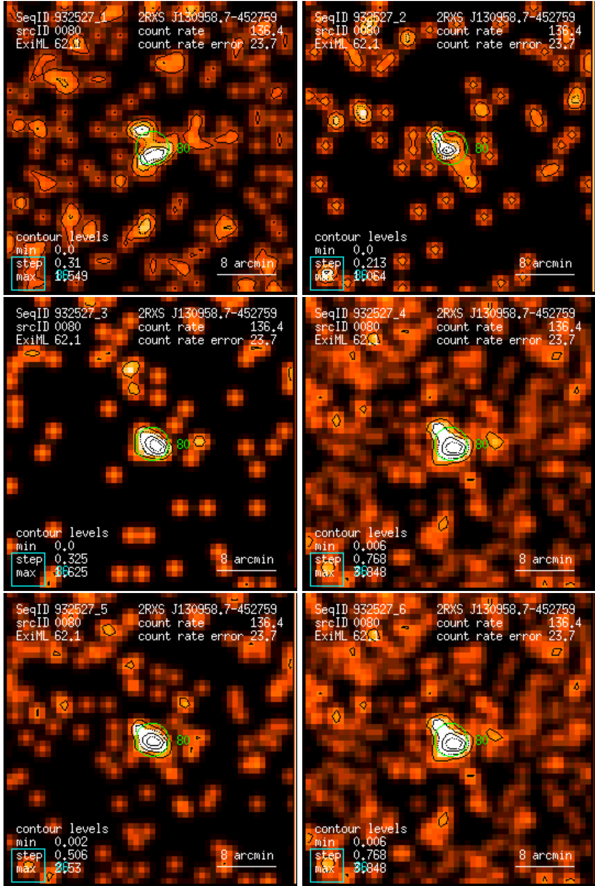
Figure 80: RASS 932527: detection 0080: band rate images, Gaussian filter: (1) PSPC channels 11 – 41, (2) 52 – 90, (3) 91 – 201, (4) 11 – 235, (5) 52 – 201, (6) 11 – 201. Broad band rates in counts/ks. Band rate contour levels in counts/ks/arcmin 2 .
