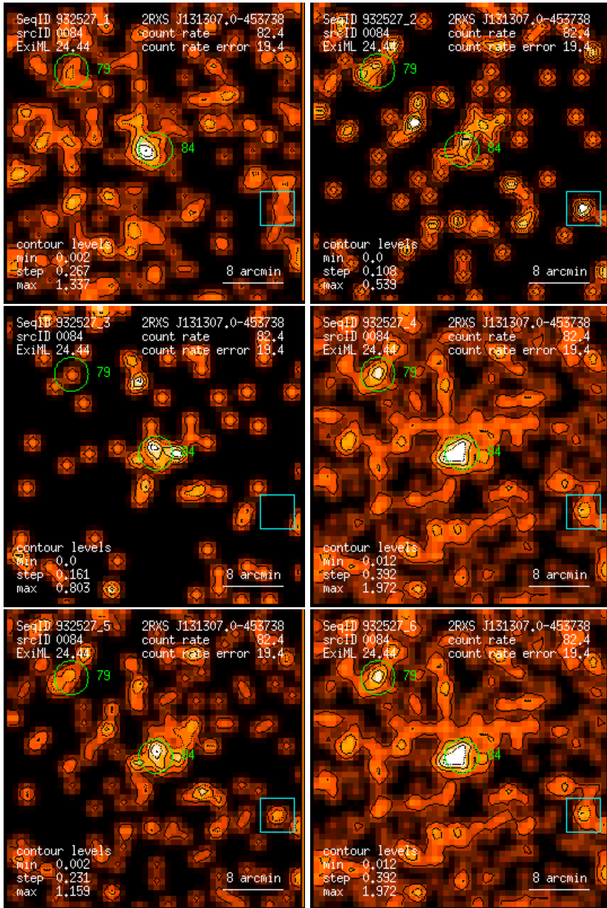
Figure 84: RASS 932527: detection 0084: band rate images, Gaussian filter: (1) PSPC channels 11 – 41, (2) 52 – 90, (3) 91 – 201, (4) 11 – 235, (5) 52 – 201, (6) 11 – 201. Broad band rates in counts/ks. Band rate contour levels in counts/ks/arcmin 2 .
