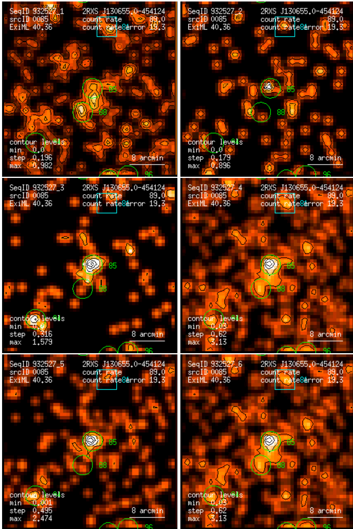
Figure 85: RASS 932527: detection 0085: band rate images, Gaussian filter: (1) PSPC channels 11 – 41, (2) 52 – 90, (3) 91 – 201, (4) 11 – 235, (5) 52 – 201, (6) 11 – 201. Broad band rates in counts/ks. Band rate contour levels in counts/ks/arcmin 2 .
