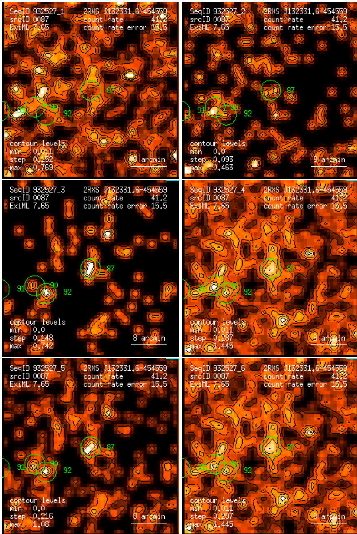
Figure 87: RASS 932527: detection 0087: band rate images, Gaussian filter: (1) PSPC channels 11 – 41, (2) 52 – 90, (3) 91 – 201, (4) 11 – 235, (5) 52 – 201, (6) 11 – 201. Broad band rates in counts/ks. Band rate contour levels in counts/ks/arcmin 2 .
