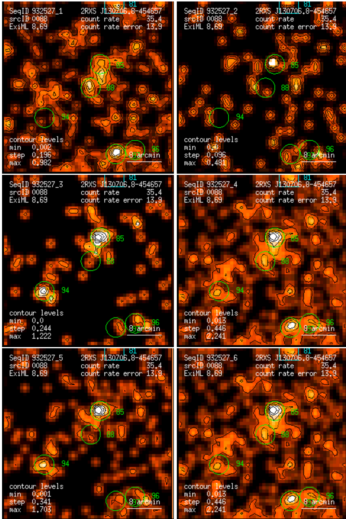
Figure 88: RASS 932527: detection 0088: band rate images, Gaussian filter: (1) PSPC channels 11 – 41, (2) 52 – 90, (3) 91 – 201, (4) 11 – 235, (5) 52 – 201, (6) 11 – 201. Broad band rates in counts/ks. Band rate contour levels in counts/ks/arcmin 2 .
