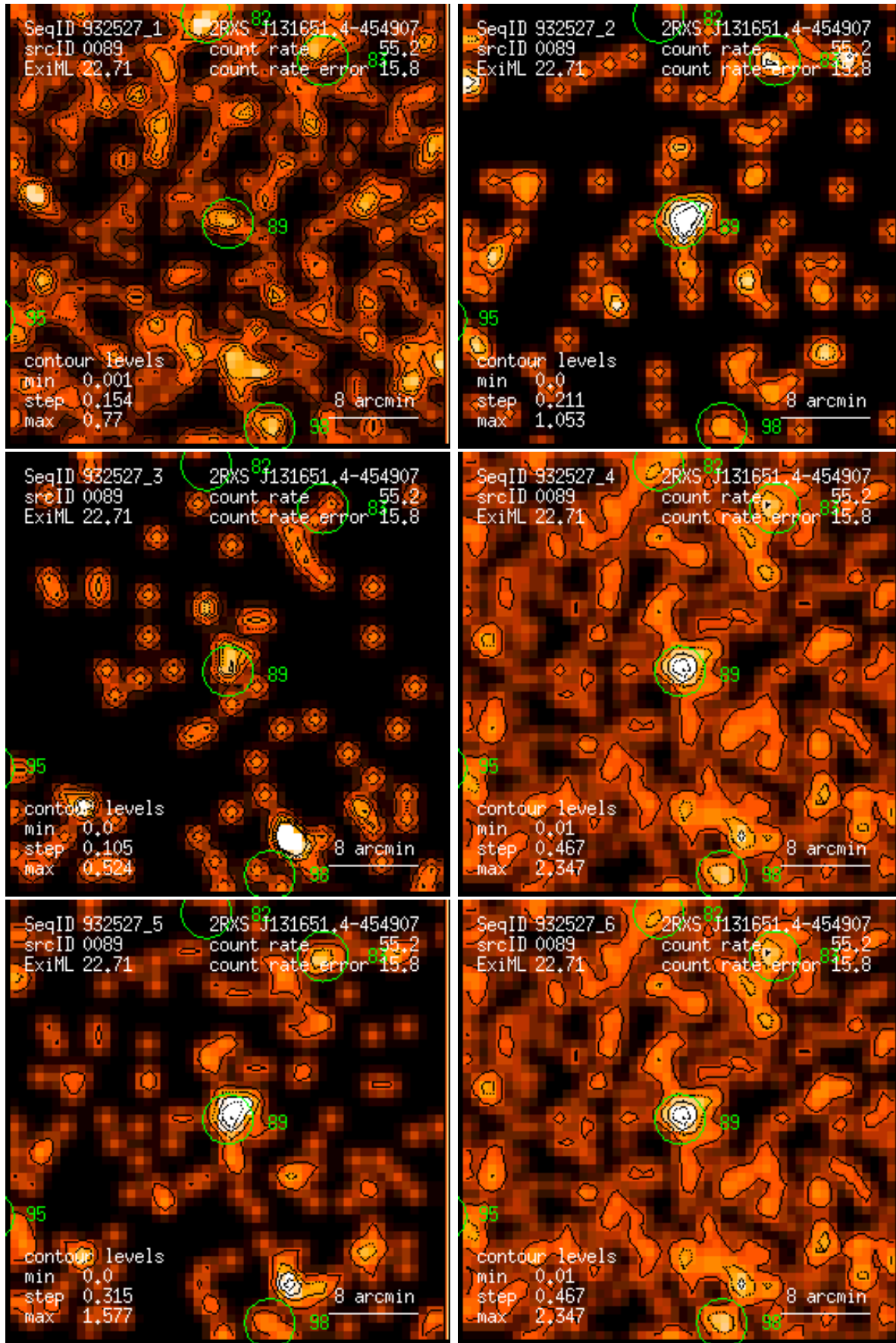
Figure 89: RASS 932527: detection 0089: band rate images, Gaussian filter: (1) PSPC channels 11 – 41, (2) 52 – 90, (3) 91 – 201, (4) 11 – 235, (5) 52 – 201, (6) 11 – 201. Broad band rates in counts/ks. Band rate contour levels in counts/ks/arcmin 2 .
