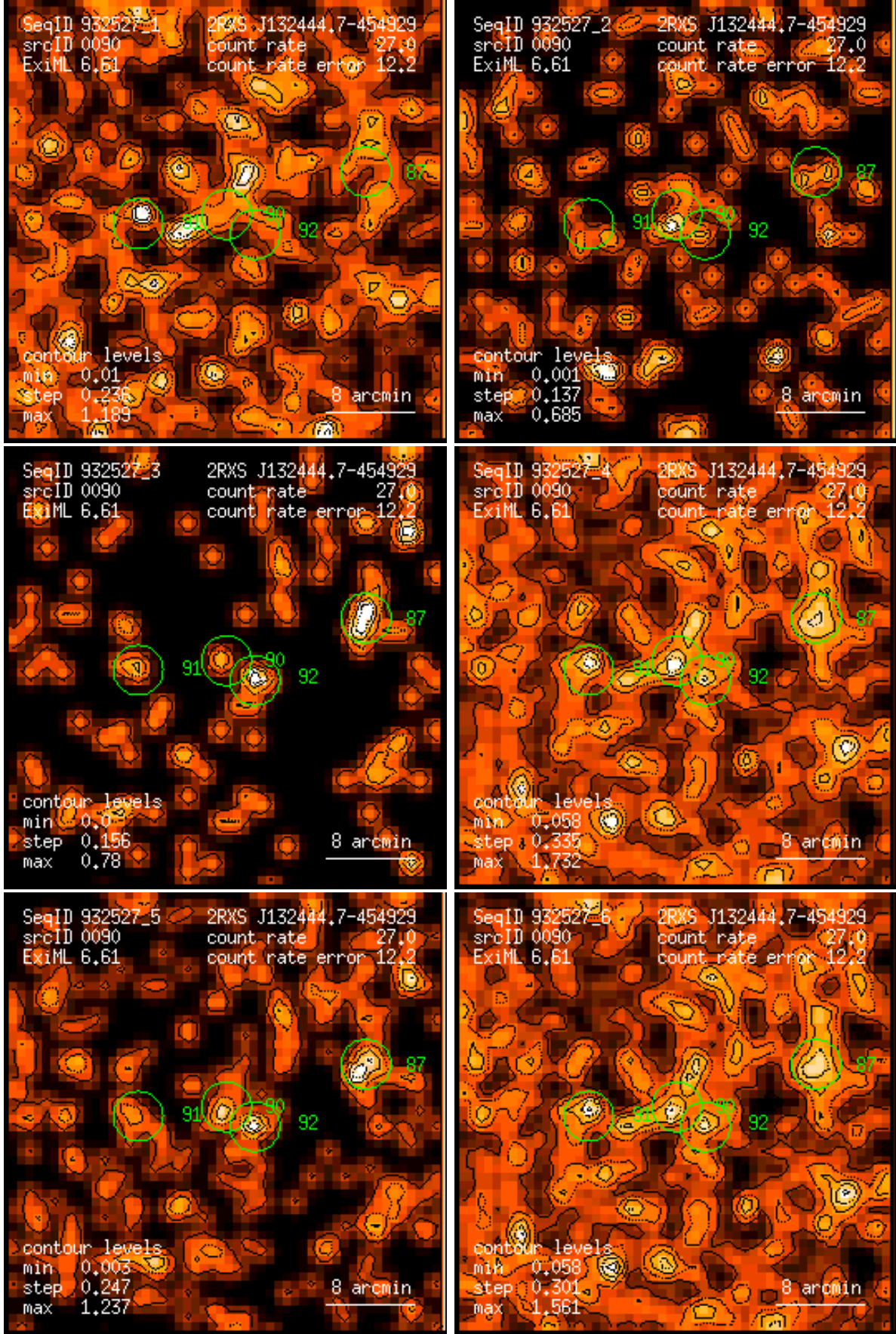
Figure 90: RASS 932527: detection 0090: band rate images, Gaussian filter: (1) PSPC channels 11 – 41, (2) 52 – 90, (3) 91 – 201, (4) 11 – 235, (5) 52 – 201, (6) 11 – 201. Broad band rates in counts/ks. Band rate contour levels in counts/ks/arcmin 2 .
