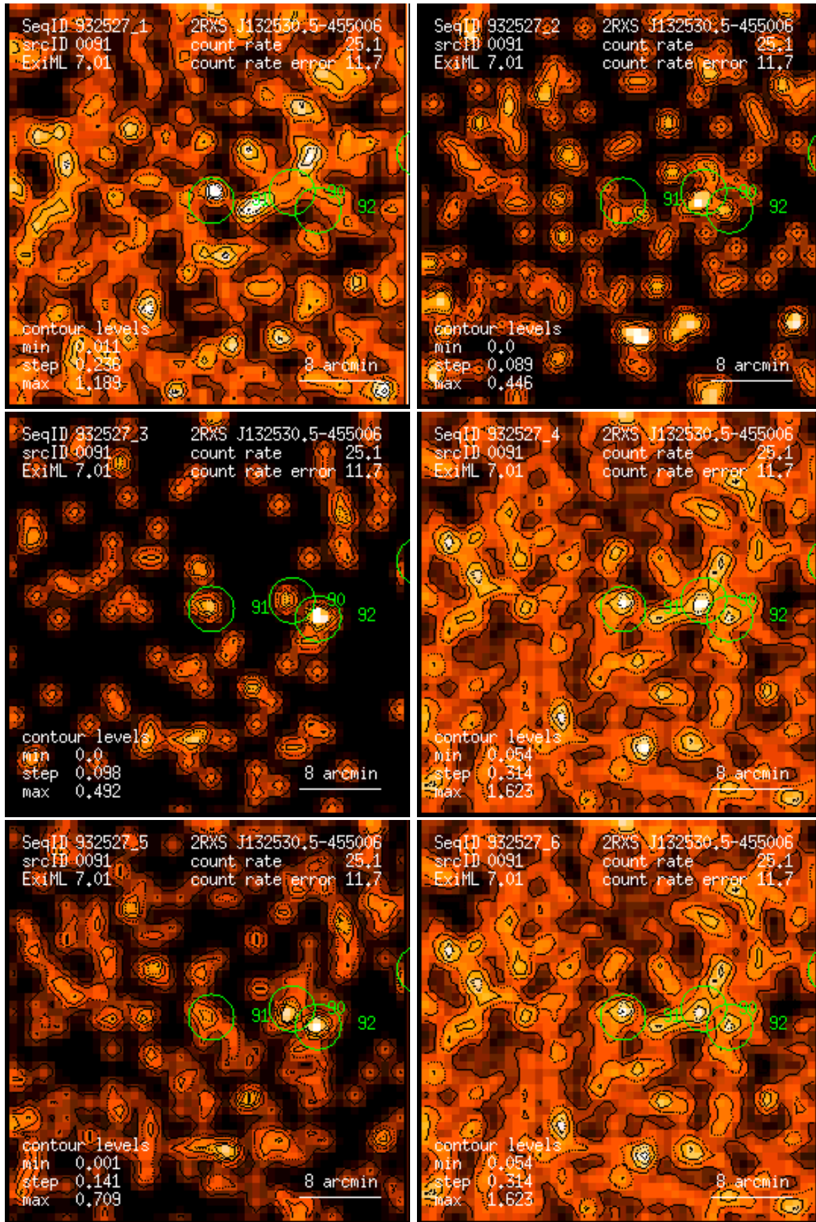
Figure 91: RASS 932527: detection 0091: band rate images, Gaussian filter: (1) PSPC channels 11 – 41, (2) 52 – 90, (3) 91 – 201, (4) 11 – 235, (5) 52 – 201, (6) 11 – 201. Broad band rates in counts/ks. Band rate contour levels in counts/ks/arcmin 2 .
