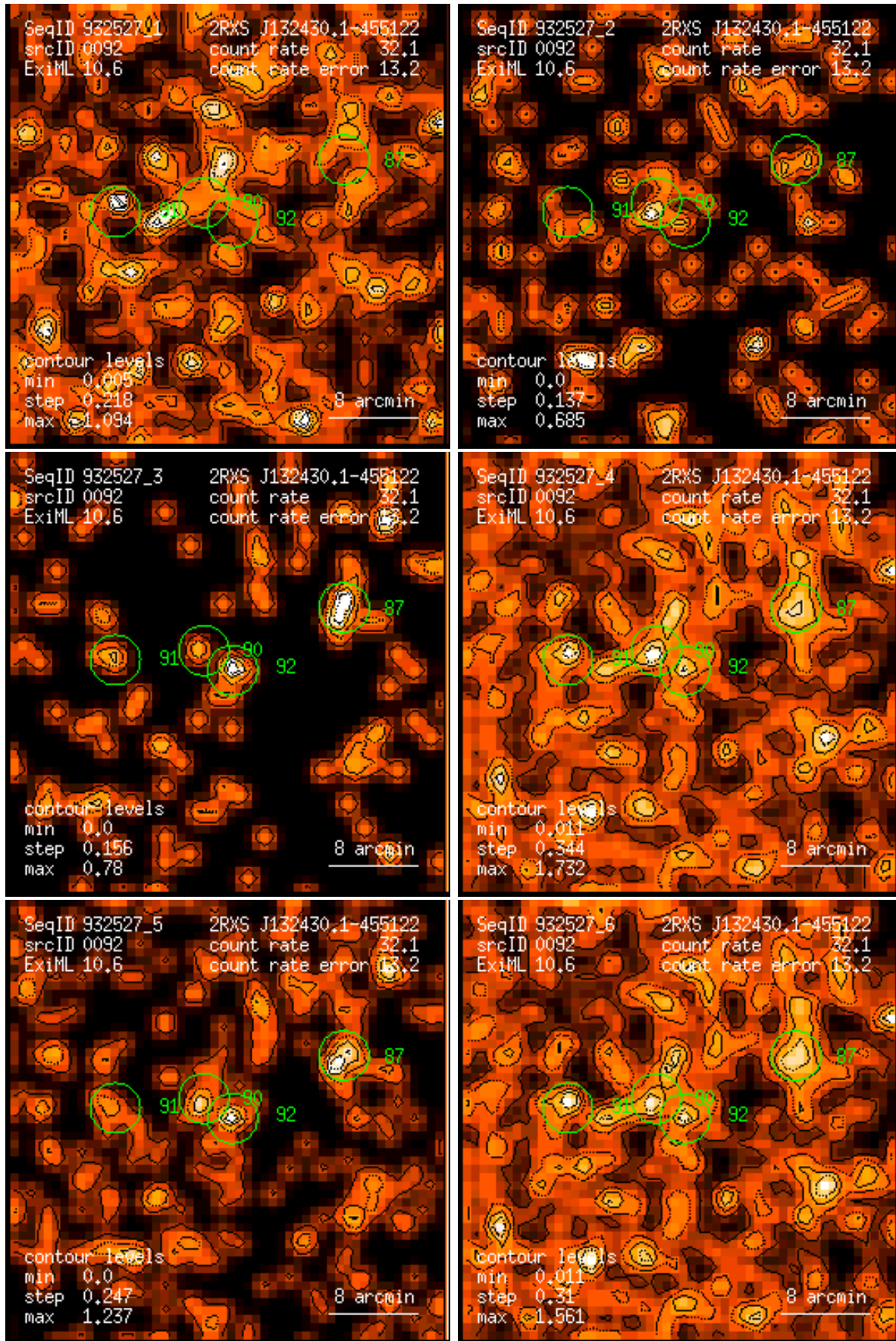
Figure 92: RASS 932527: detection 0092: band rate images, Gaussian filter: (1) PSPC channels 11 – 41, (2) 52 – 90, (3) 91 – 201, (4) 11 – 235, (5) 52 – 201, (6) 11 – 201. Broad band rates in counts/ks. Band rate contour levels in counts/ks/arcmin 2 .
