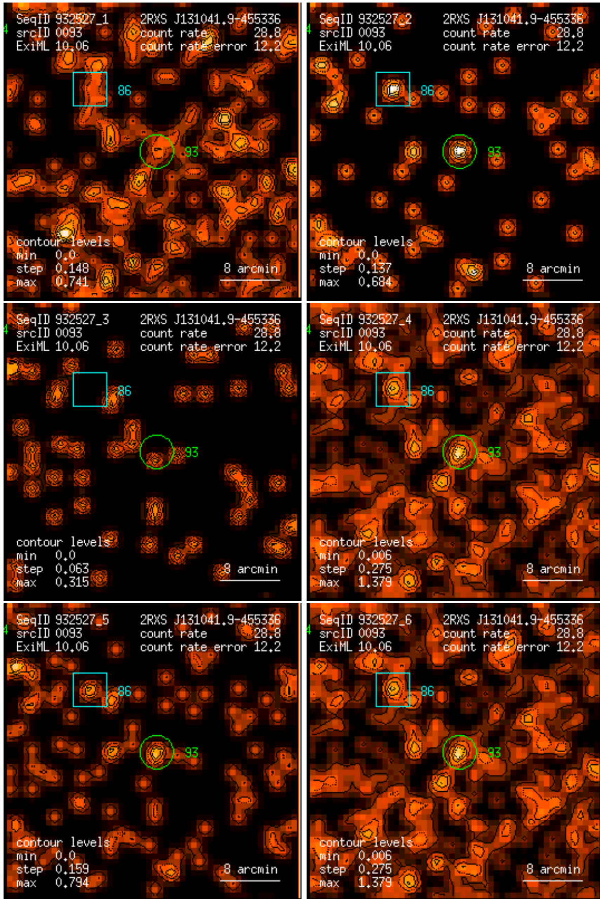
Figure 93: RASS 932527: detection 0093: band rate images, Gaussian filter: (1) PSPC channels 11 – 41, (2) 52 – 90, (3) 91 – 201, (4) 11 – 235, (5) 52 – 201, (6) 11 – 201. Broad band rates in counts/ks. Band rate contour levels in counts/ks/arcmin 2 .
