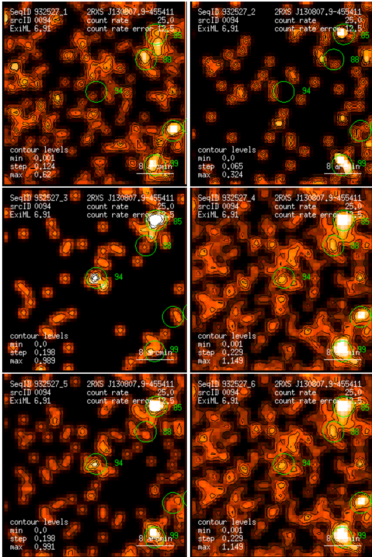
Figure 94: RASS 932527: detection 0094: band rate images, Gaussian filter: (1) PSPC channels 11 – 41, (2) 52 – 90, (3) 91 – 201, (4) 11 – 235, (5) 52 – 201, (6) 11 – 201. Broad band rates in counts/ks. Band rate contour levels in counts/ks/arcmin 2 .
