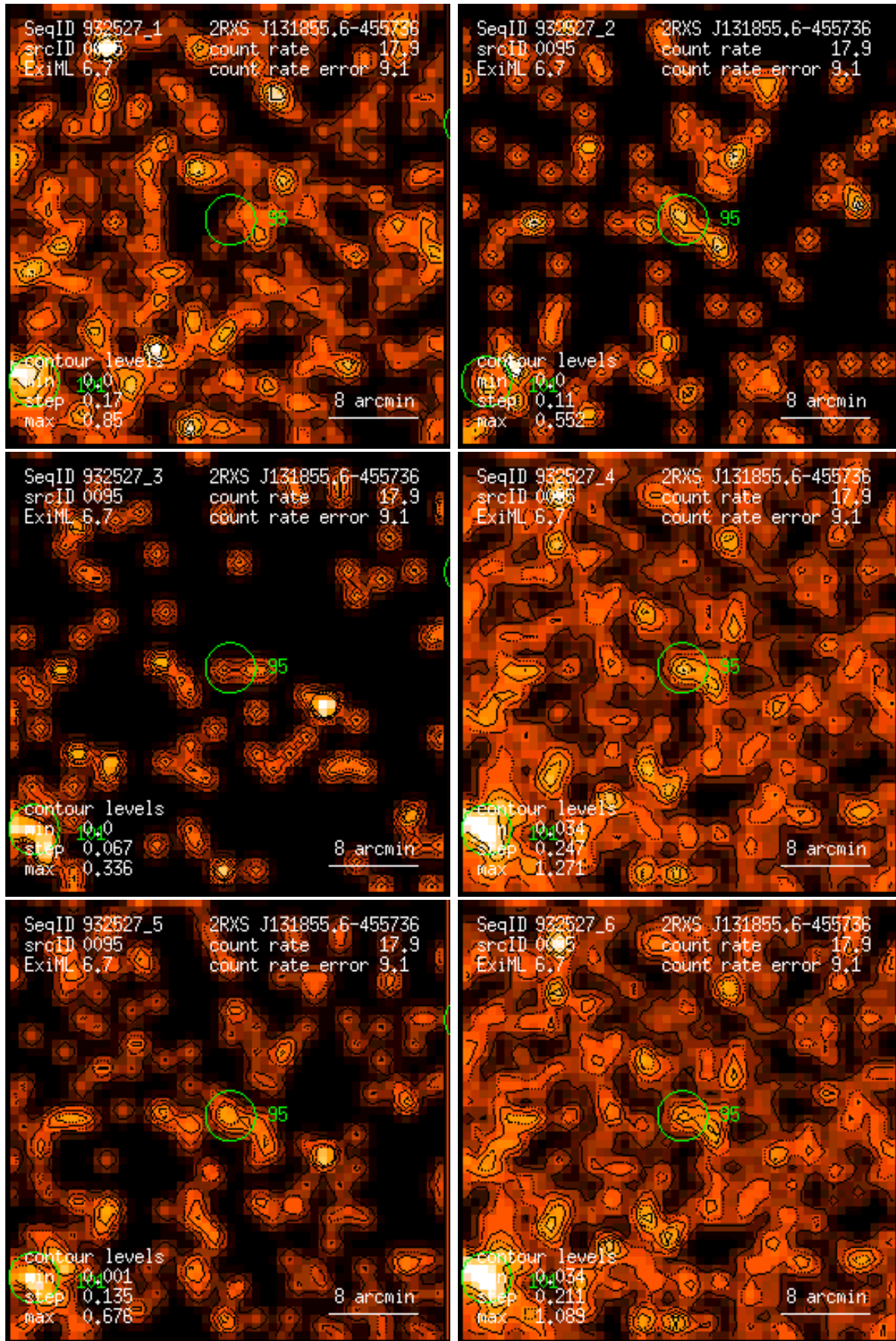
Figure 95: RASS 932527: detection 0095: band rate images, Gaussian filter: (1) PSPC channels 11 – 41, (2) 52 – 90, (3) 91 – 201, (4) 11 – 235, (5) 52 – 201, (6) 11 – 201. Broad band rates in counts/ks. Band rate contour levels in counts/ks/arcmin 2 .
