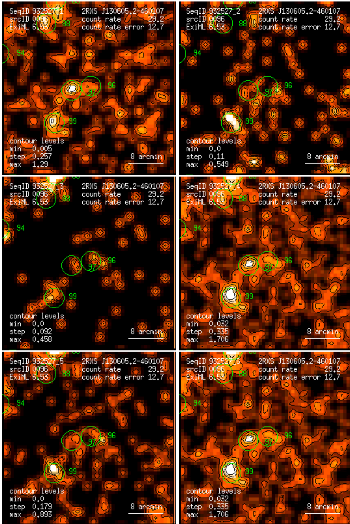
Figure 96: RASS 932527: detection 0096: band rate images, Gaussian filter: (1) PSPC channels 11 – 41, (2) 52 – 90, (3) 91 – 201, (4) 11 – 235, (5) 52 – 201, (6) 11 – 201. Broad band rates in counts/ks. Band rate contour levels in counts/ks/arcmin 2 .
