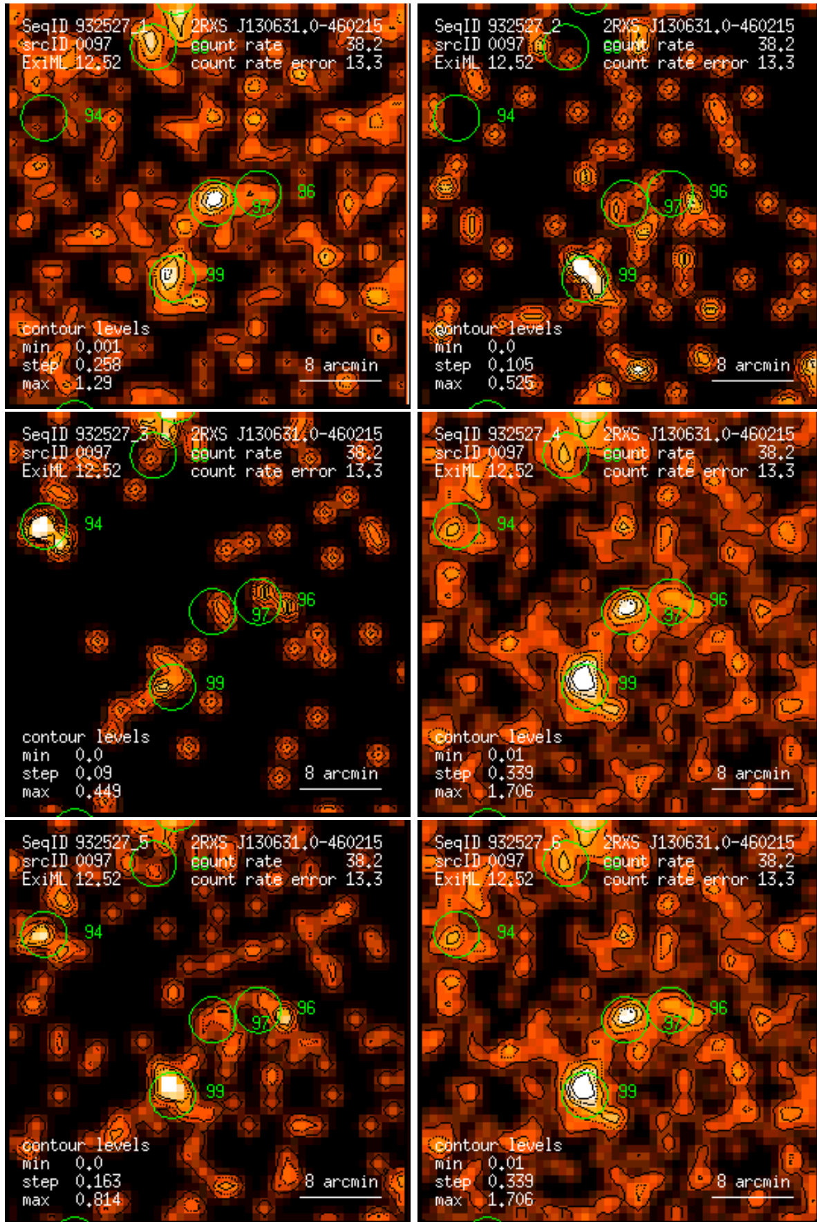
Figure 97: RASS 932527: detection 0097: band rate images, Gaussian filter: (1) PSPC channels 11 – 41, (2) 52 – 90, (3) 91 – 201, (4) 11 – 235, (5) 52 – 201, (6) 11 – 201. Broad band rates in counts/ks. Band rate contour levels in counts/ks/arcmin 2 .
