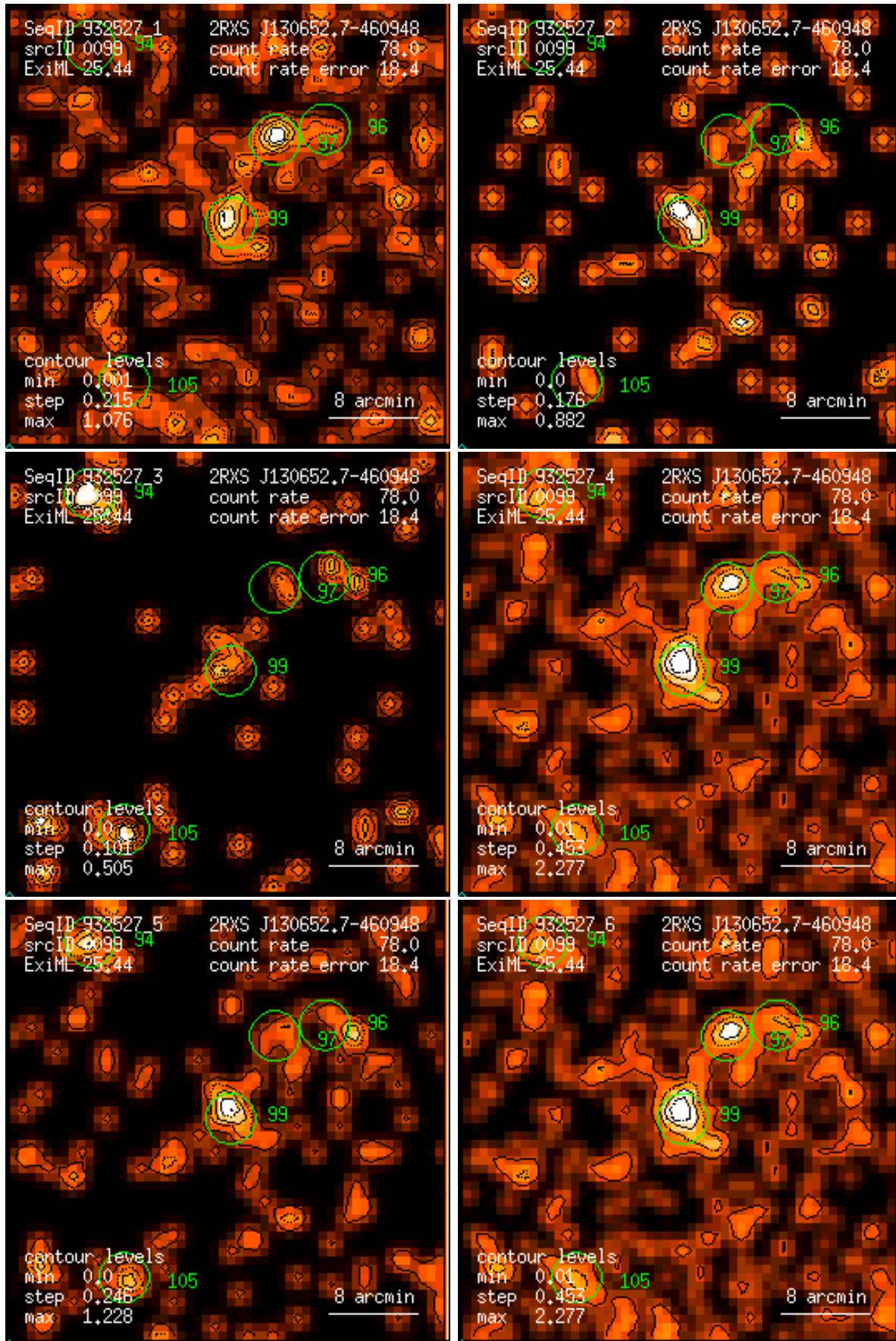
Figure 99: RASS 932527: detection 0099: band rate images, Gaussian filter: (1) PSPC channels 11 – 41, (2) 52 – 90, (3) 91 – 201, (4) 11 – 235, (5) 52 – 201, (6) 11 – 201. Broad band rates in counts/ks. Band rate contour levels in counts/ks/arcmin 2 .
