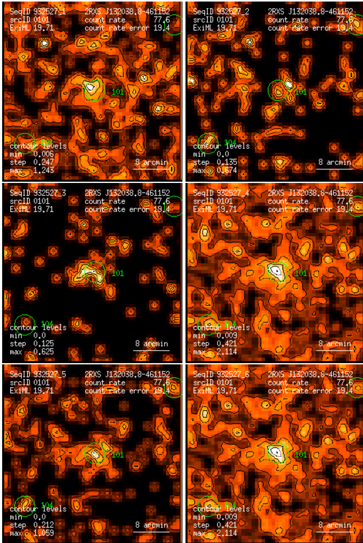
Figure 101: RASS 932527: detection 0101: band rate images, Gaussian filter: (1) PSPC channels 11 – 41, (2) 52 – 90, (3) 91 – 201, (4) 11 – 235, (5) 52 – 201, (6) 11 – 201. Broad band rates in counts/ks. Band rate contour levels in counts/ks/arcmin 2 .
