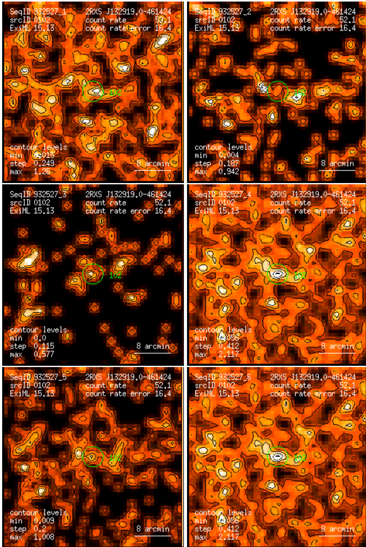
Figure 102: RASS 932527: detection 0102: band rate images, Gaussian filter: (1) PSPC channels 11 – 41, (2) 52 – 90, (3) 91 – 201, (4) 11 – 235, (5) 52 – 201, (6) 11 – 201. Broad band rates in counts/ks. Band rate contour levels in counts/ks/arcmin 2 .
