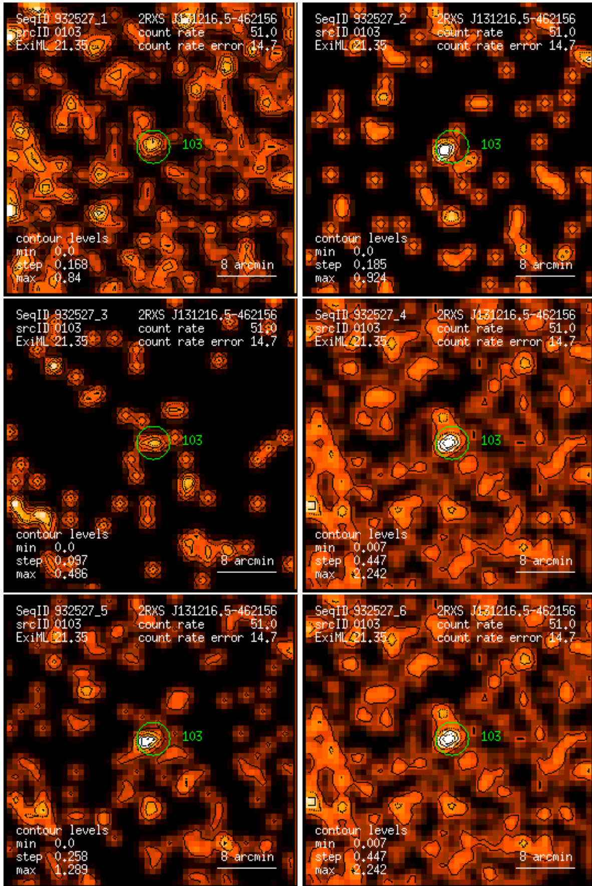
Figure 103: RASS 932527: detection 0103: band rate images, Gaussian filter: (1) PSPC channels 11 – 41, (2) 52 – 90, (3) 91 – 201, (4) 11 – 235, (5) 52 – 201, (6) 11 – 201. Broad band rates in counts/ks. Band rate contour levels in counts/ks/arcmin 2 .
