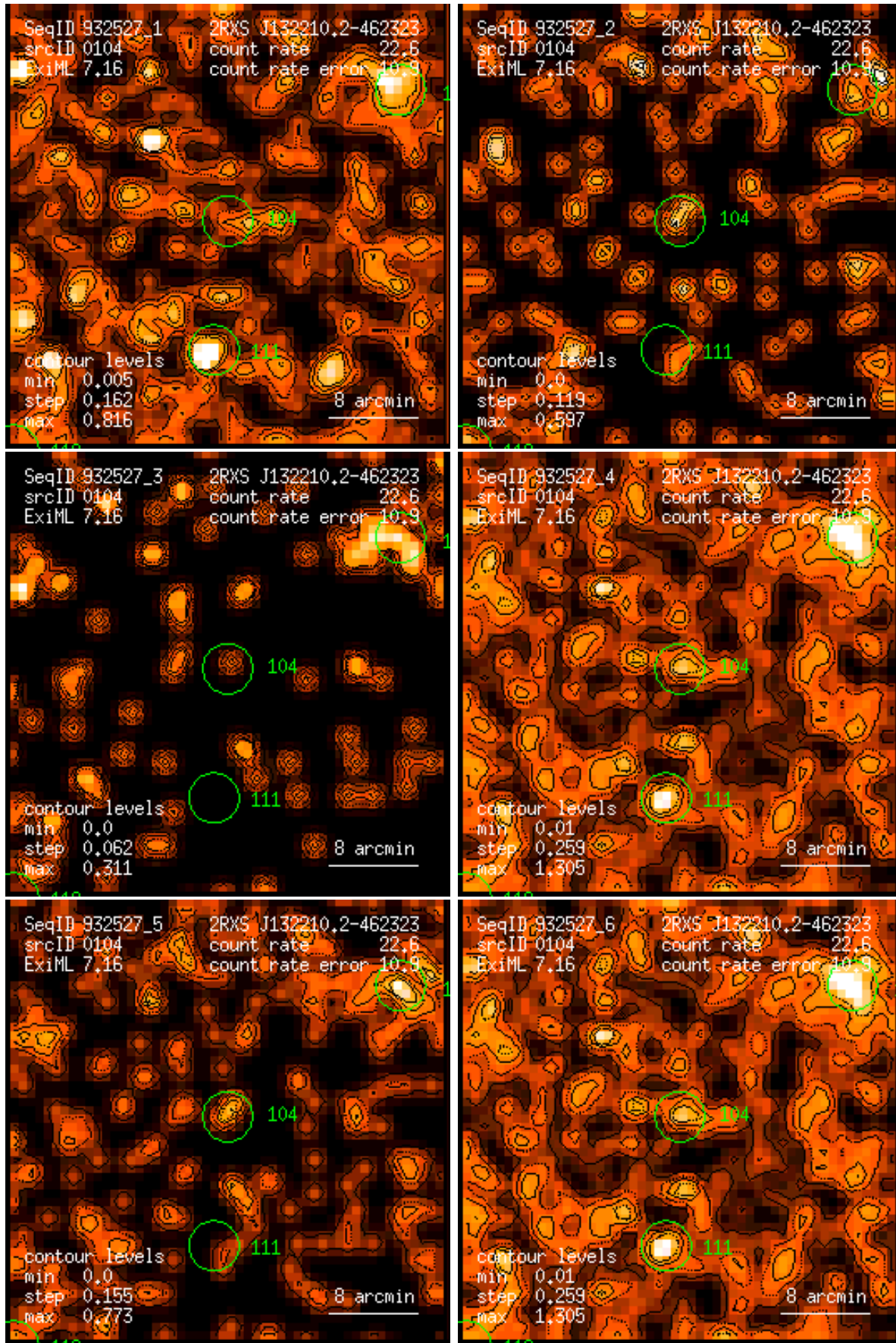
Figure 104: RASS 932527: detection 0104: band rate images, Gaussian filter: (1) PSPC channels 11 – 41, (2) 52 – 90, (3) 91 – 201, (4) 11 – 235, (5) 52 – 201, (6) 11 – 201. Broad band rates in counts/ks. Band rate contour levels in counts/ks/arcmin 2 .
